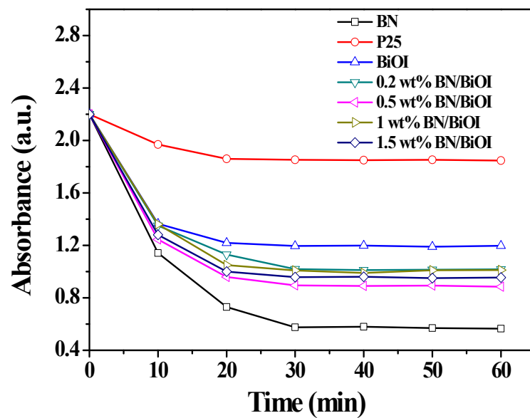
Fig. S2 The adsorption equilibrium curves of different samples for RhB over 60 min.
