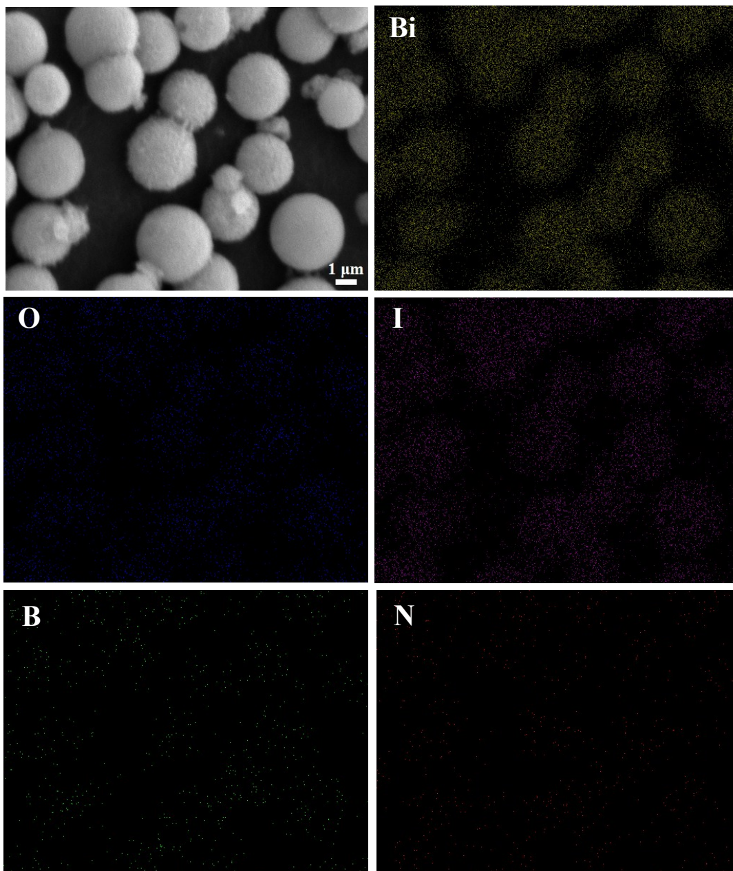
Fig. S1 Typical SEM image of 0.5 wt% BN/BiOI composite and corresponding elemental mapping images of Bi, O, I, B and N.
