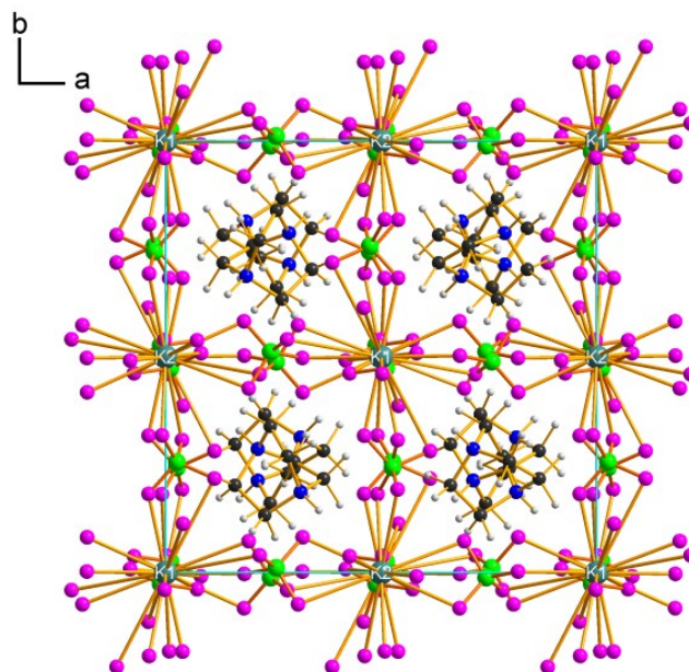
Fig. S2 The representation of the cell packing viewed along the cell axis. Colour scheme: \text{K}^+ , teal; O, pink; Cl, green; C, black; N, blue; H, gray.
