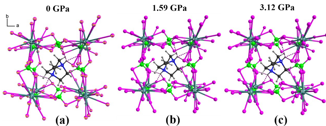
Fig. S1 The representation of the unit cell of [\text{DABCOH}_2^{2+}][\text{K}(\text{ClO}_4)_3] viewed along the cell axis, at 0 (a), 1.59 (b) and 3.12 GPa (c), refined from DFT based on experimental cell parameters. Colour scheme: \text{K}^+ , teal; O, pink; Cl, green; C, black; N, blue; H, gray. N–H \cdots O bonds are represented as dashed purple lines.
