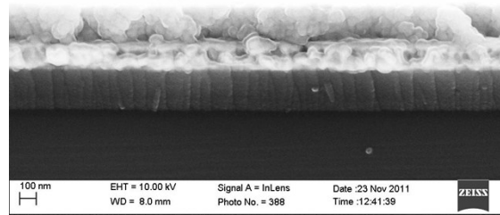
Fig. S2 Cross-sectional FE-SEM images of NF-PT thin films
