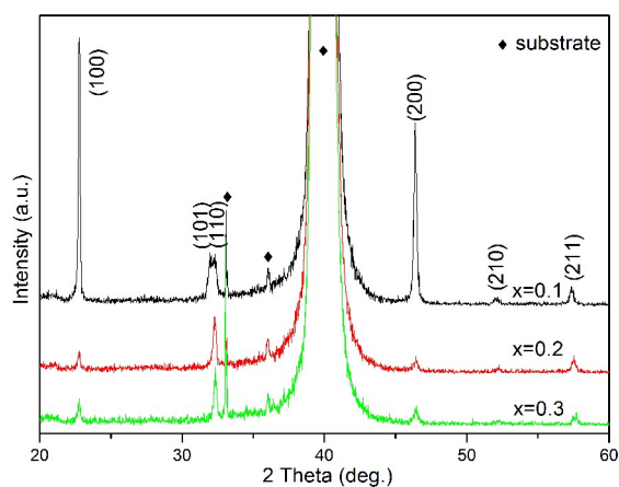
Fig. S1 Conventional powder XRD patterns of NF-PT thin films.
