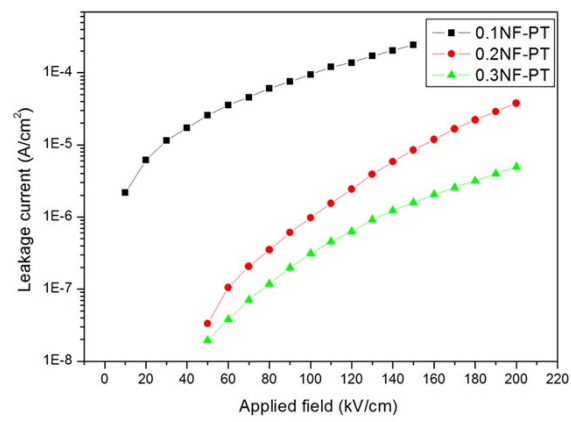
Fig. S3 Leakage current intensity of NF-PT thin films
