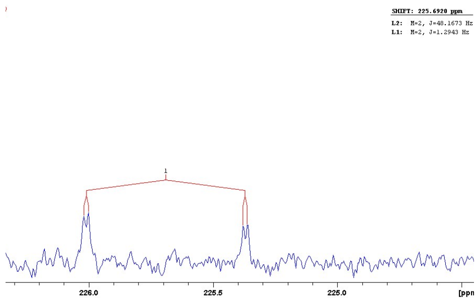
Figure 4. Selected portion of ^{13}\text{C} NMR spectrum of 7 in \text{CDCl}_3
