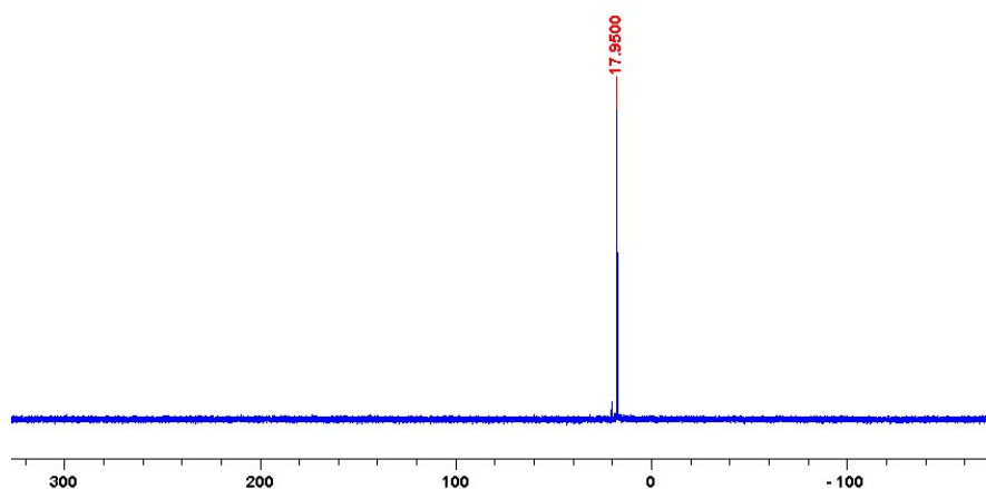
Figure.3 ^{31}\text{P}\{^1\text{H}\} NMR spectrum of 7 in \text{CDCl}_3
