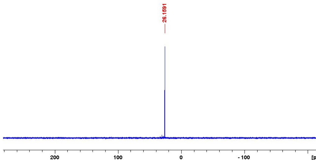
Figure.1 ^{31}\text{P}\{^1\text{H}\} NMR spectrum of 6 in \text{D}_2\text{O}
