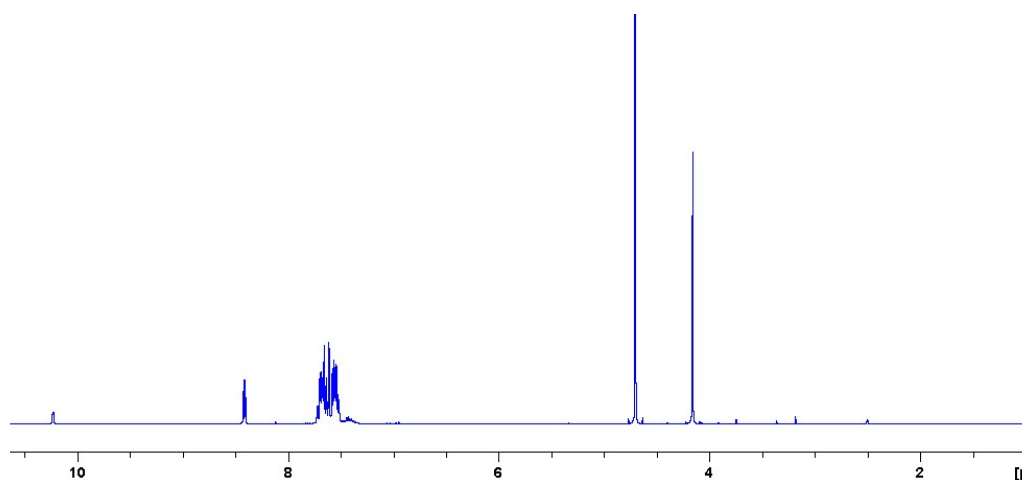
Figure.2 ^1\text{H} NMR spectrum of 6 in \text{D}_2\text{O}
