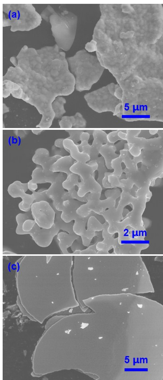
Fig. S1 SEM images of (a) L-Ni 2 P, (b) L-Co 2 P and (c) L-MoP.
