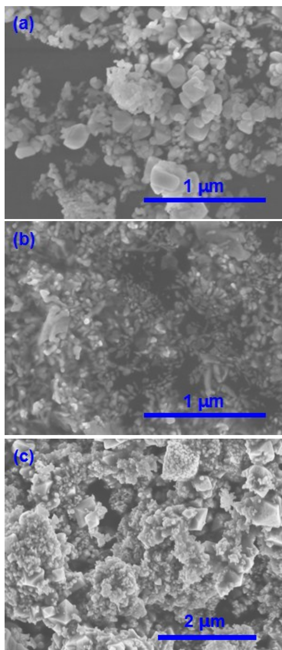
Fig. S2 SEM images of (a) NiO, (b) \text{Co}_3\text{O}_4 and (c) \text{MoO}_3 .
