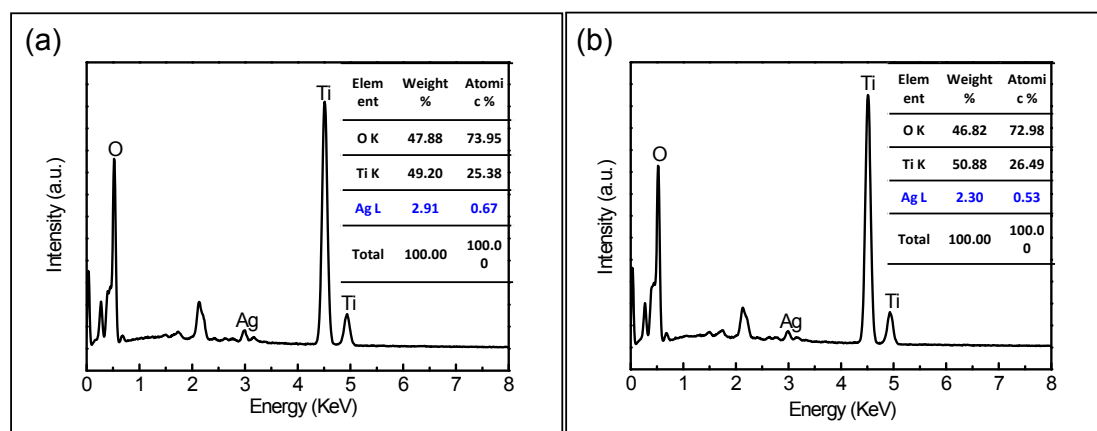
Fig. S1 EDX spectra of Ti-90/Ag 2 NCN before (a) and after (b) photocatalytic experiments
