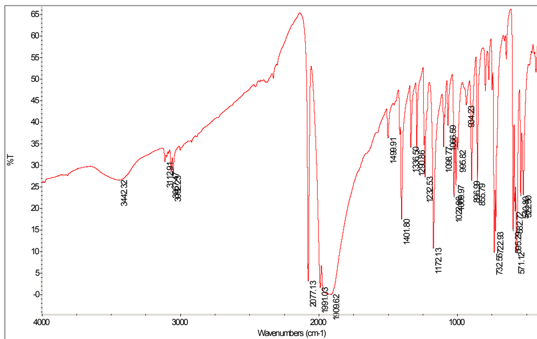
Compound 2g
