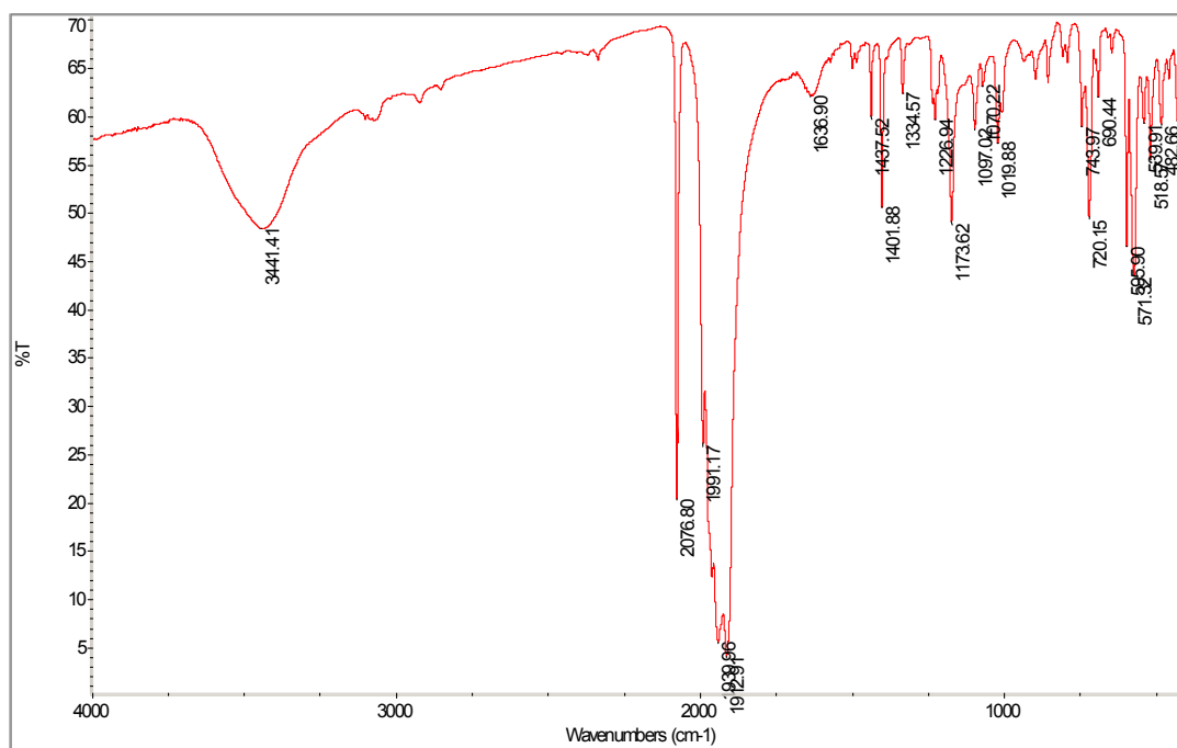
Compound 2f
