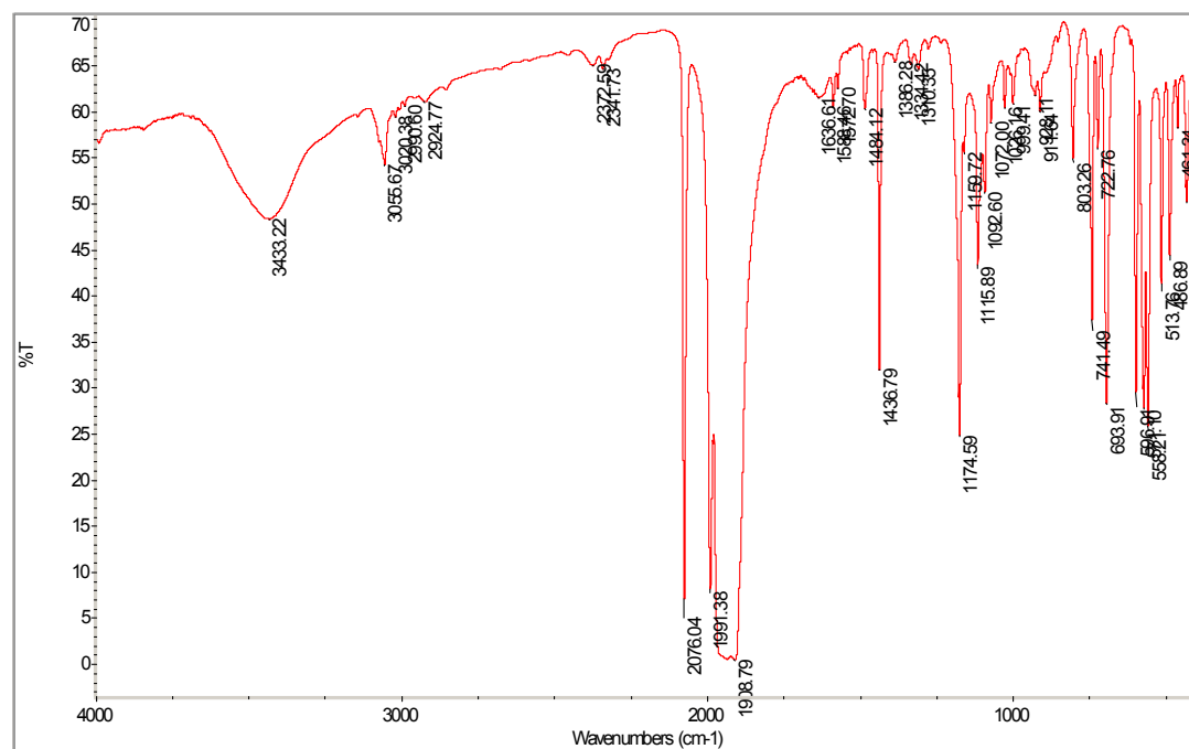
Compound 2a-2
