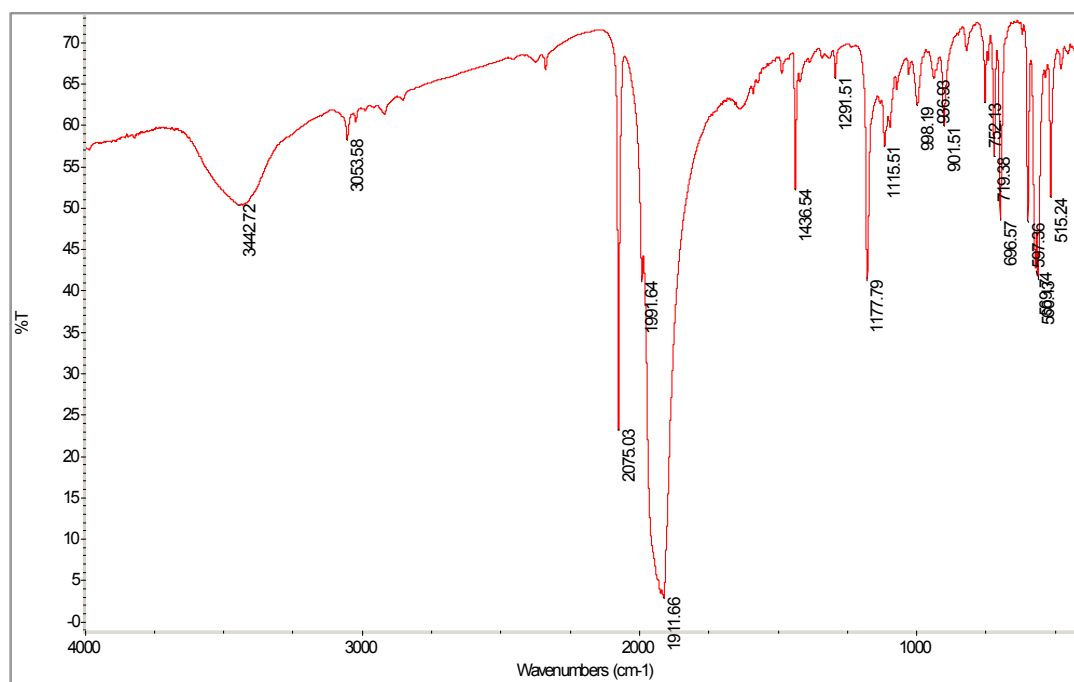
Compound 2b
