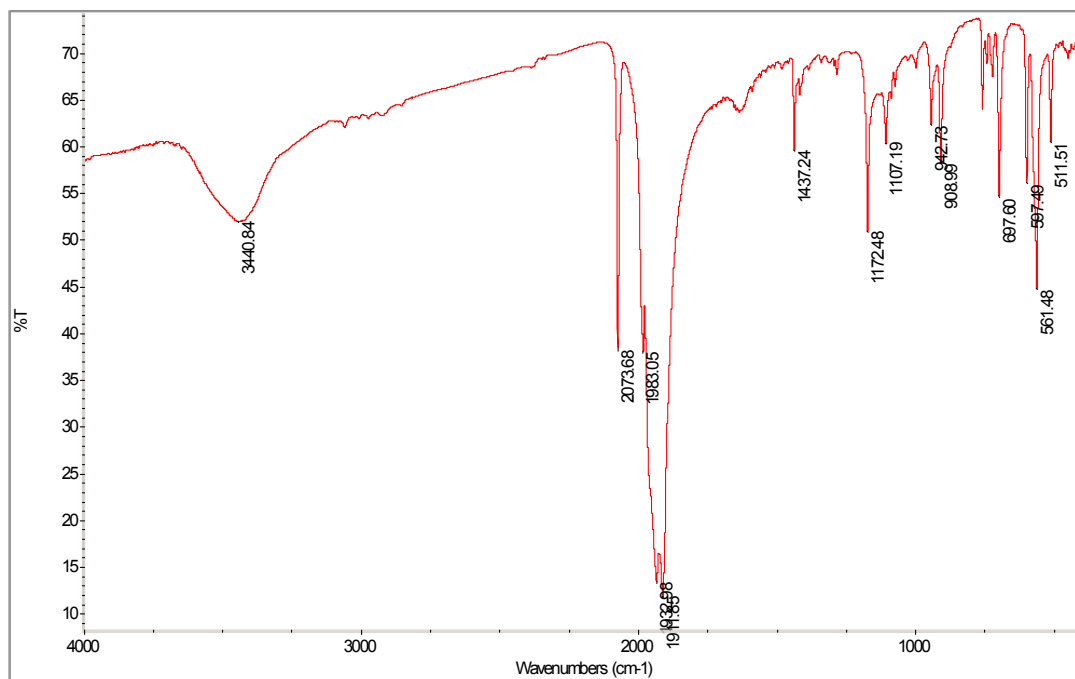
Compound 4
