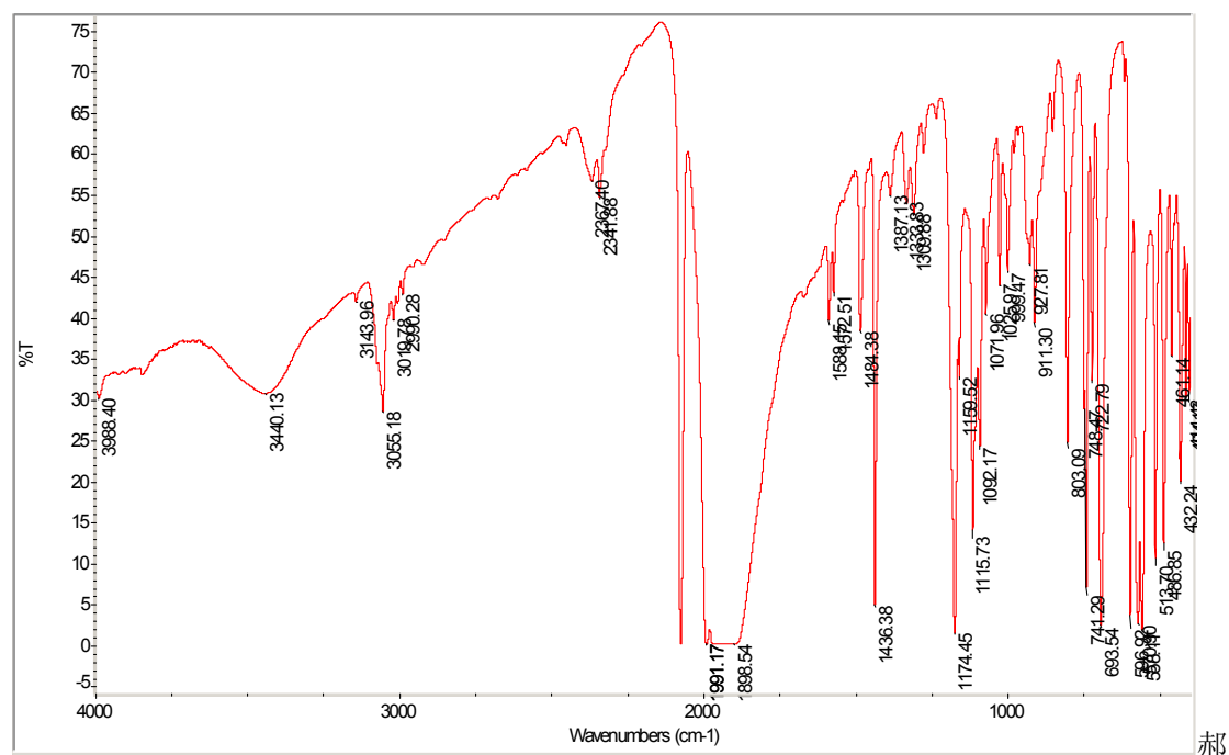
Compound 2a
