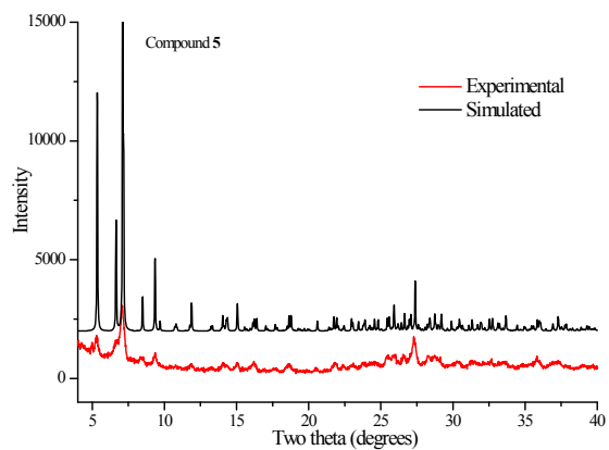
Fig. s2 experimental and simulated XRD patterns of compounds 1-5.
