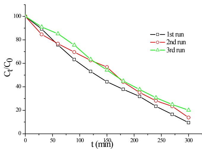
Fig. s7 Repeated catalytic experiments results of RhB.
