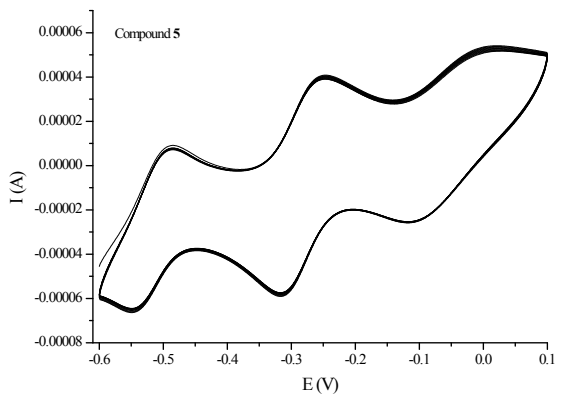
Fig. s4 cyclic voltammograms of CPEs 1-5.
