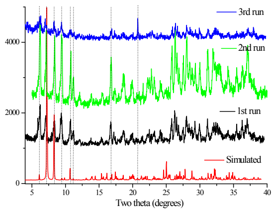
Fig. s6 the simulated and X-ray powder diffraction patterns after three runs of repeated experiments of compound 3.
