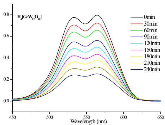
Fig. s5 photodegradation properties of H 4 [GeW 12 O 40 ].
