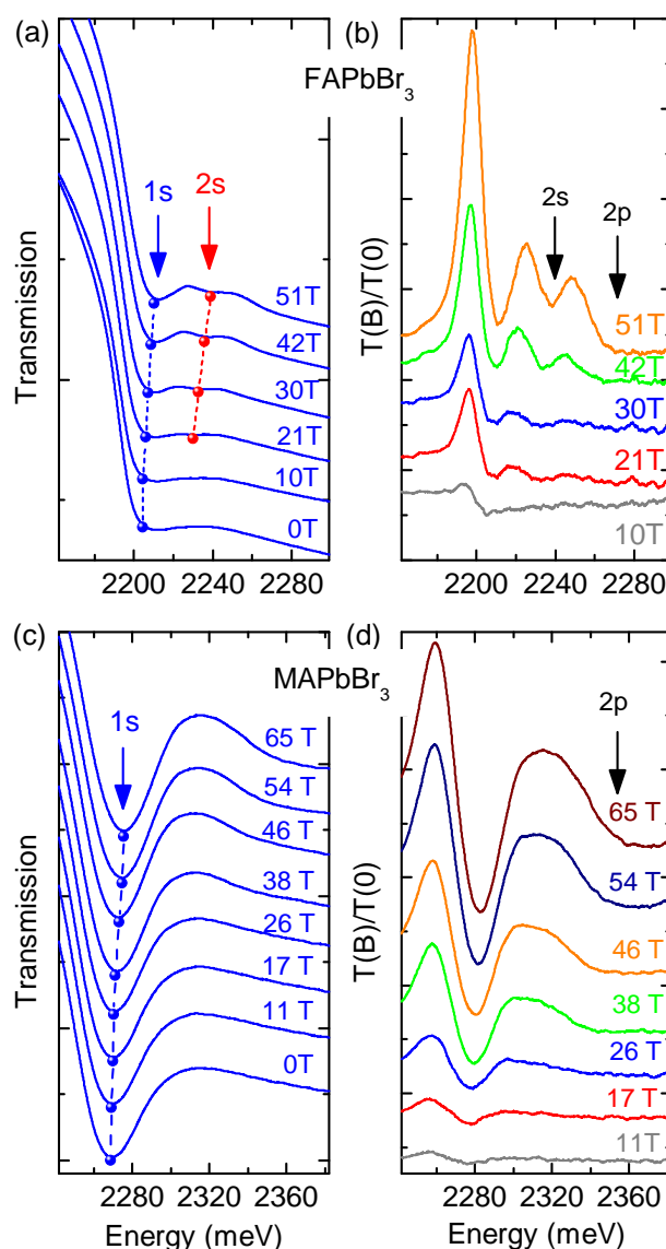
Fig. 1 Low temperature data for FAPbBr 3 and MAPbBr 3 (a), (c) transmission spectra for different magnetic fields, (b), (d) transmission spectra at fixed field ratioed to the zero field spectrum.
