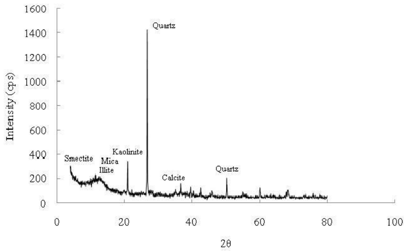
Figure A2. X-Ray Diffraction (XRD) of sediment samples (a) 1C_50
