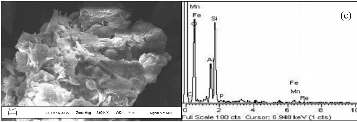
Figure A1. SEM and EDX of soil sediment samples (a) C_50 (b) C_70 (c) 1C_150.
