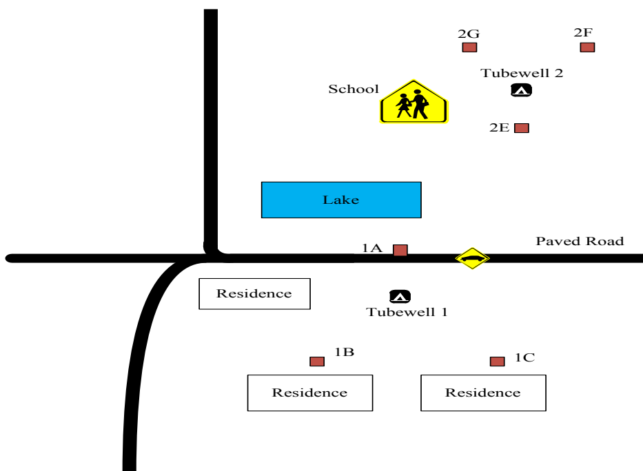
Fig A1: Showing the site location of drilling in higher As contaminated Tube-wells 1 and 2.
