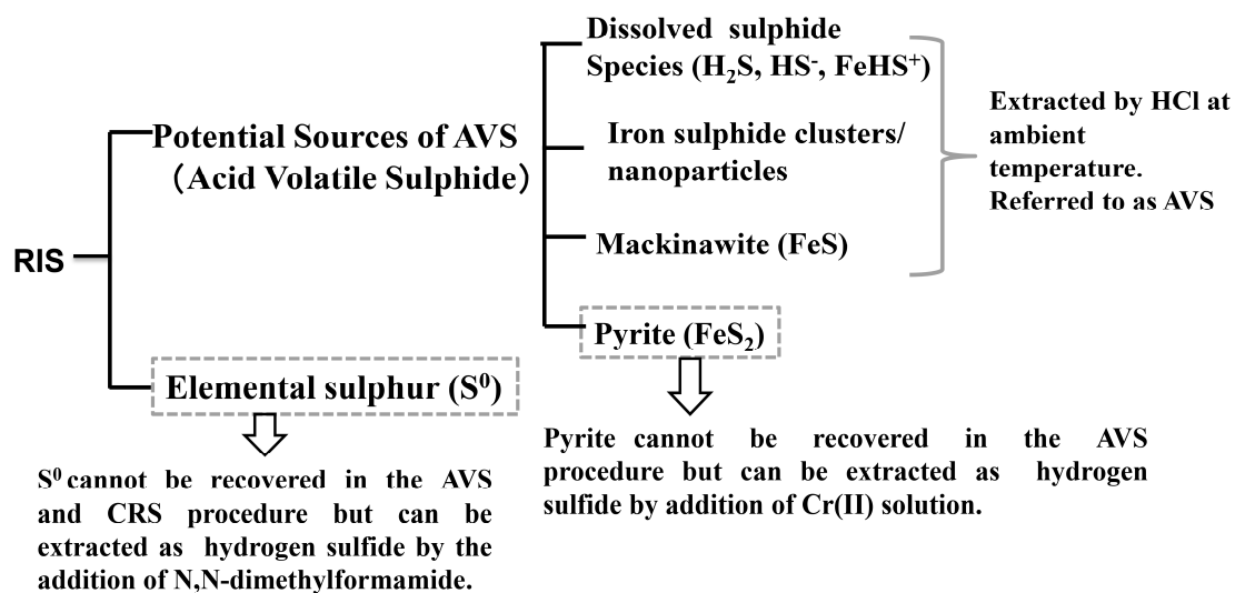
Fig. S2 Analysis of the extractable reduced inorganic sulphur (RIS)
