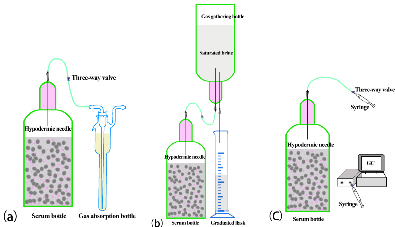
Fig. S1 Determinations of hydrogen sulphide (a), biogas volume (b) and biogas composition(c)
