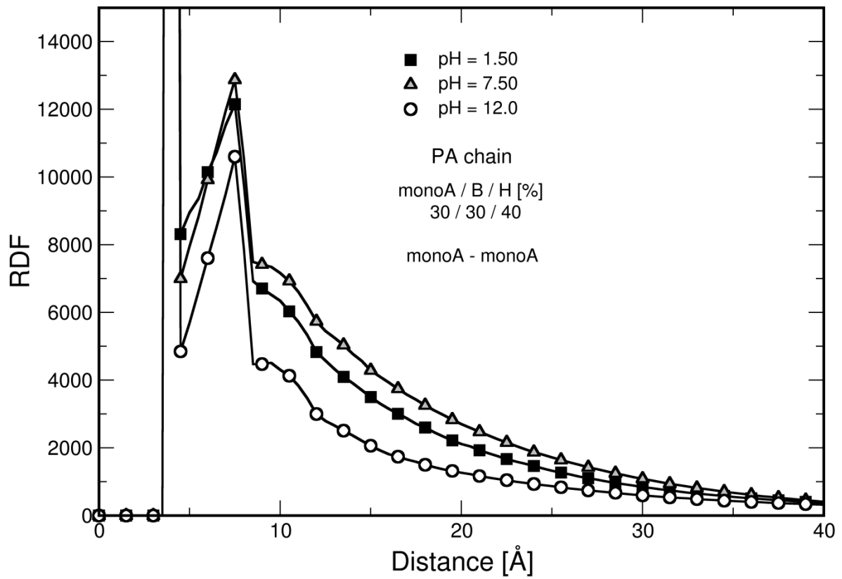
S2. Monomer A – monomer A, Radial Distribution Function of a random polymer chain at different pH values.
