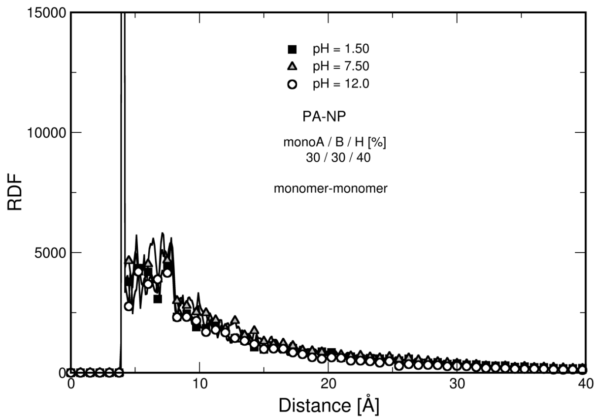
S5. Monomer – monomer, Radial Distribution Function of a random polymer chain at different pH values and in the presence of the NP.
