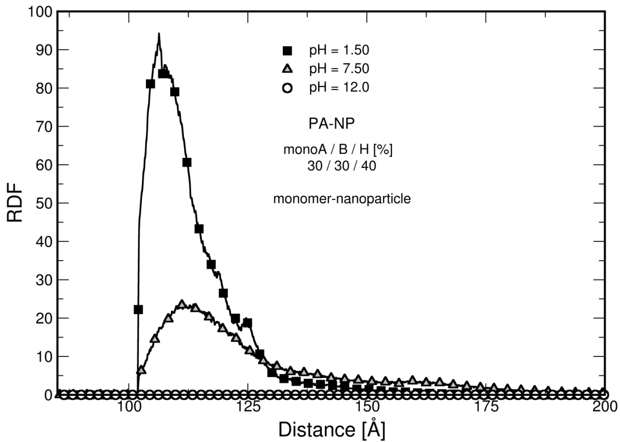
S6. Monomer – nanoparticle, Radial Distribution Function of a random polymer chain at different pH values and in the presence of the NP.
