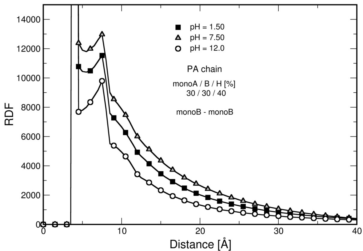
S4. Monomer B – monomer B, Radial Distribution Function of a random polymer chain at different pH values.
