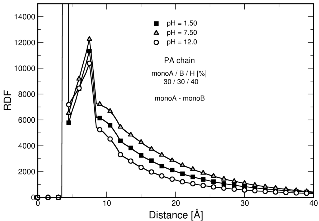
S3. Monomer A – monomer B, Radial Distribution Function of a random polymer chain at different pH values.
