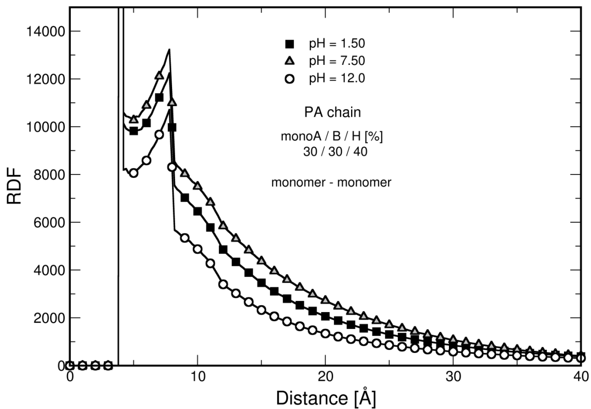
S1. Monomer – monomer Radial Distribution Function of a random polymer chain at different pH values.
