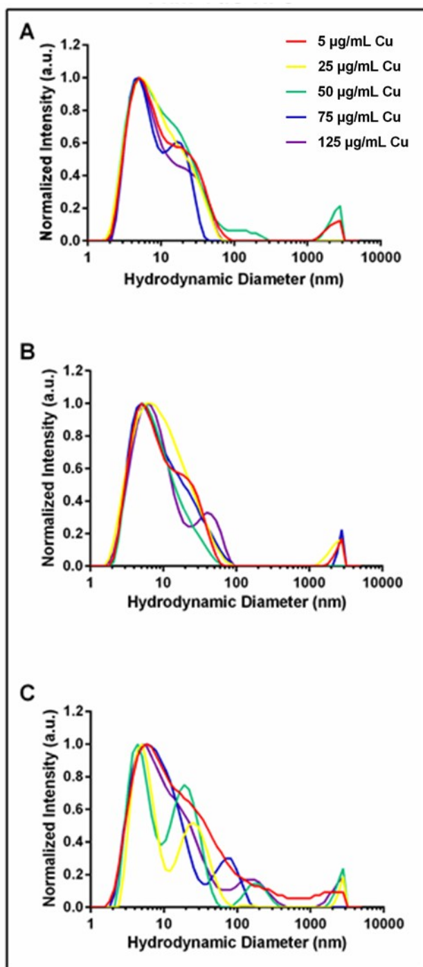
Figure 15. Distribution of hydrodynamic diameters of CuO nanoparticles (4 nm) incubated in complete medium at 37°C for 0 hours (A), 4 hours (B) and 24 hours (C).
