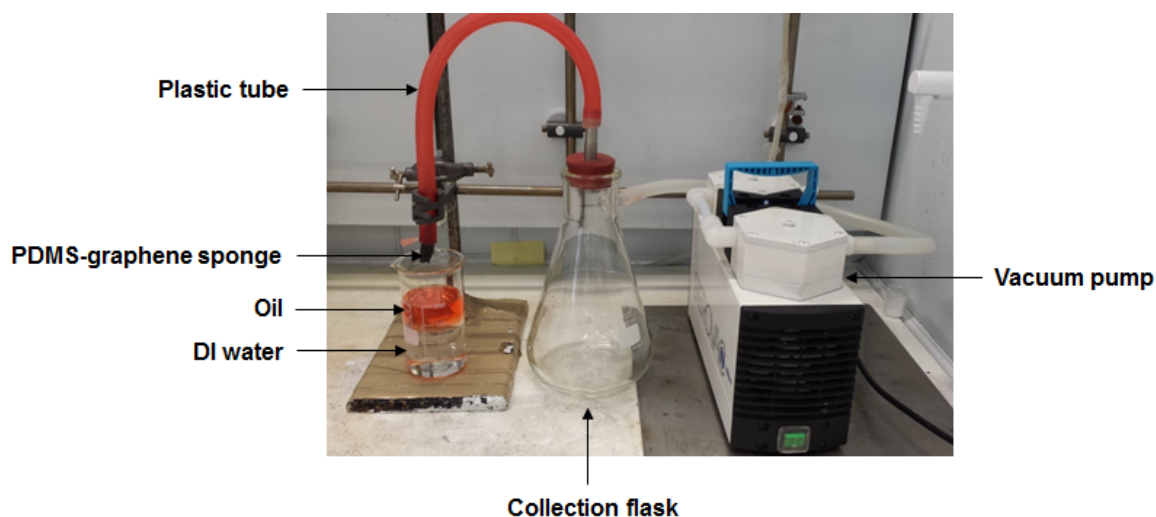
Fig. S1 Vacuum system setup for continuous oil removal from water
