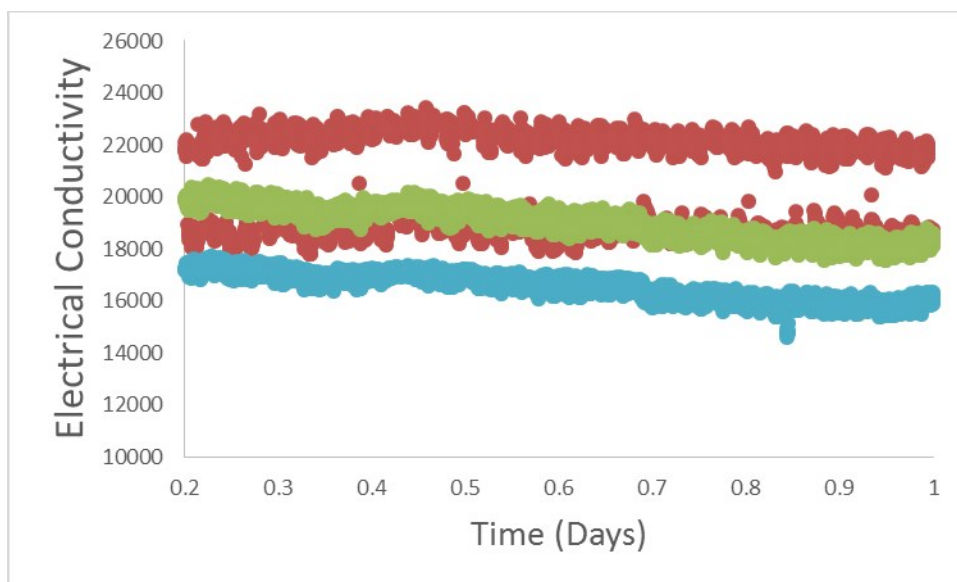
Figure S1. Change in conductivity ( \mu\text{s}/\text{cm} ) for anode, desalination and cathode chamber over the course of a day. Red icons are for desalination/regeneration of the desalination chamber, Green is for Cathode chamber and Blue correlates to the anode chamber.
