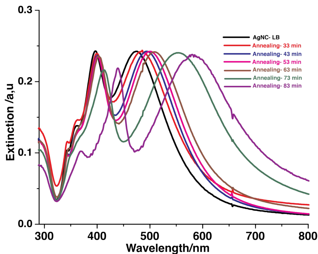
Figure S1. Optical extinction spectra of Ag NC (100 nm) embedded on PS thin-film showing red shift of dipole and quadrupolar plasmon peak upon annealing at different time.
