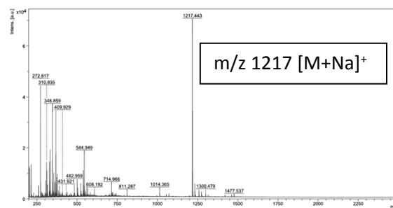
Figure S3A. MALDI-MS
