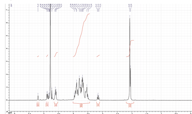
Figure S5C. 1 H NMR
