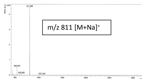
Figure S4A. MALDI-MS
