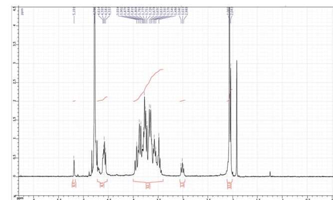
Figure S2C. 1 H NMR
