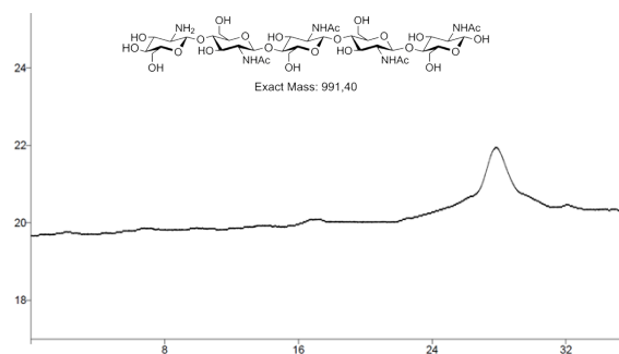
Figure S5C. 1 H NMR
