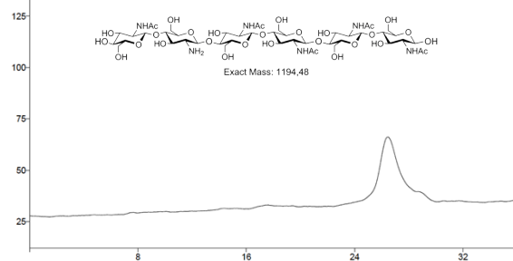
Figure S3B. HPSEC
