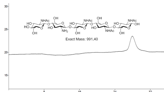
Figure S2B. HPSEC
