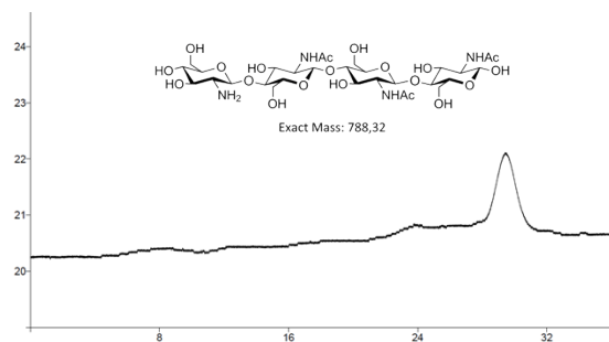
Figure S4B. HPSEC
