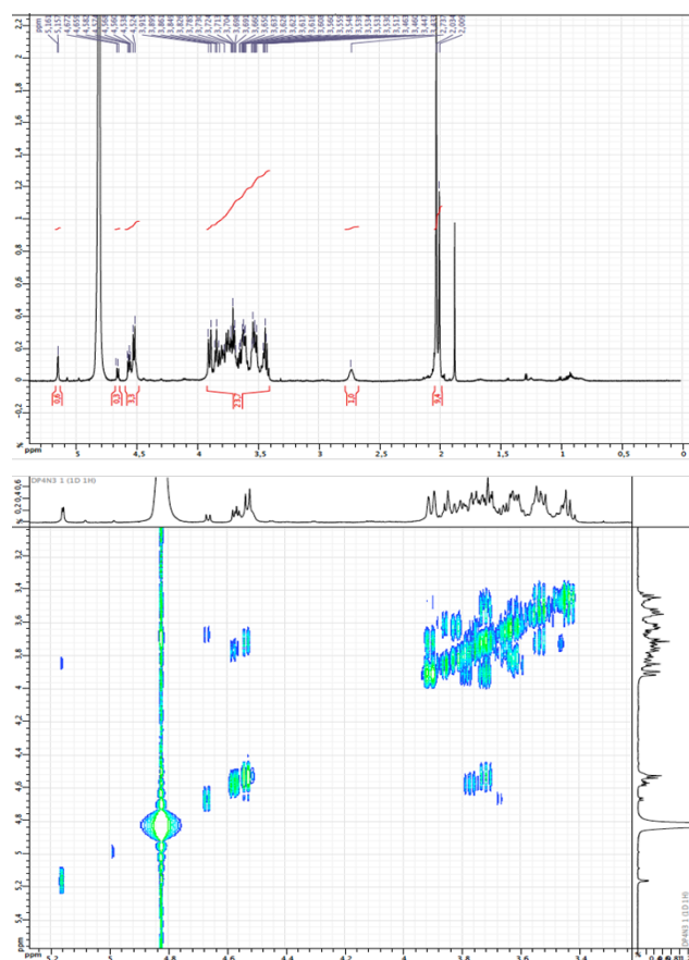
Figure S1C. 1 H NMR
