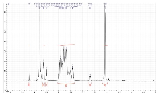
Figure S4C. 1 H NMR
