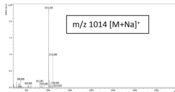
Figure S5A. MALDI-MS
