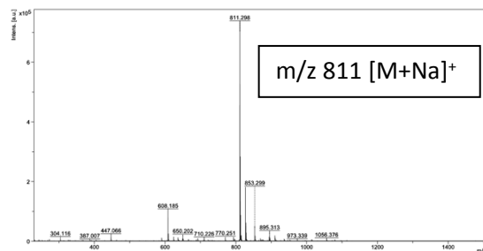
Figure S1A. MALDI-MS
