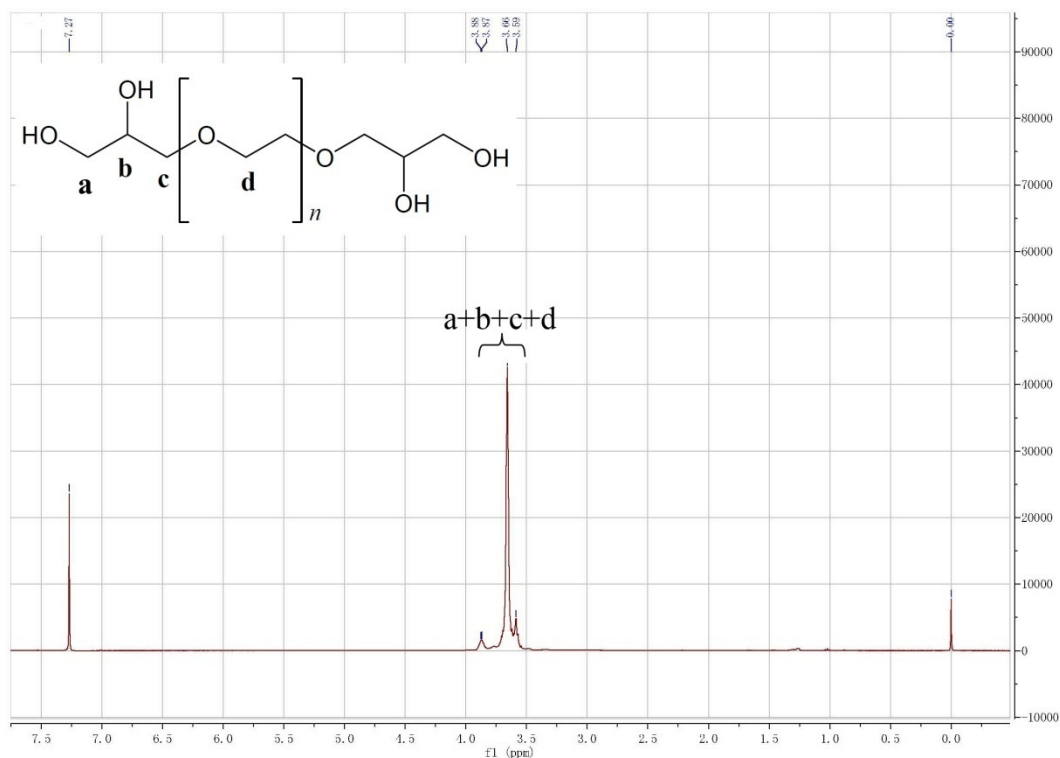
Fig. S1. ^1\text{H} NMR ( \text{CDCl}_3 , 400 MHz) of Poly(ethylene glycol) diglyceryl ether.
