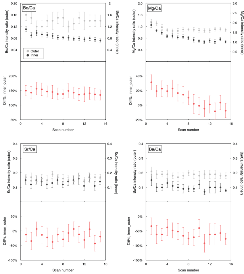
Fig. S2 Alkaline earth metal composition depth profiles.
