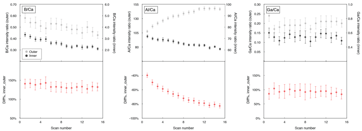
Fig. S3 B-Al-Ga composition depth profiles.
