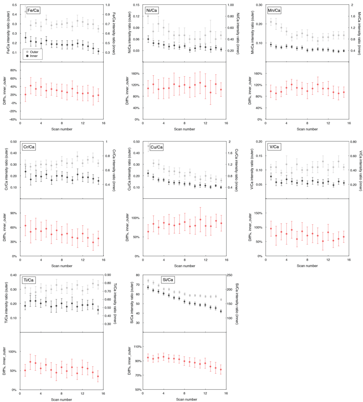
Fig. S4 Transition metal and Si composition depth profiles.
