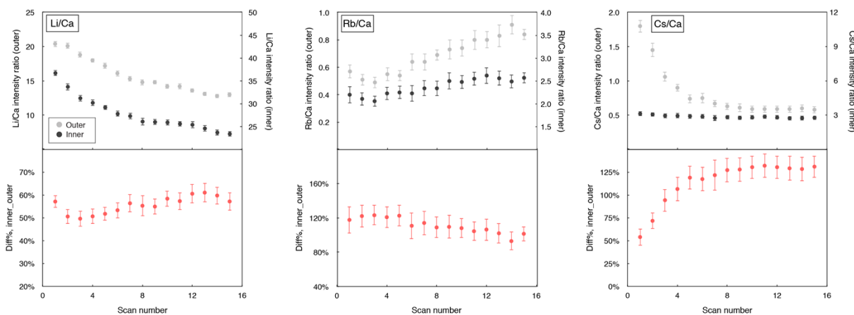
Fig. S1 Alkaline metal composition depth profiles.
