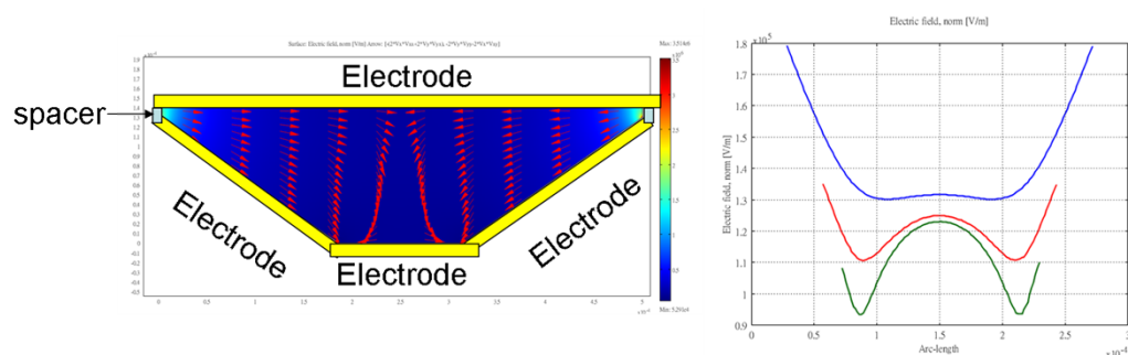
Figure S1 Finite element simulation of electric field for 3D trapezoid electrode configuration. The design of the trapezoid channel shows that the electric field distribution has two second minima field regions near the lower line.
