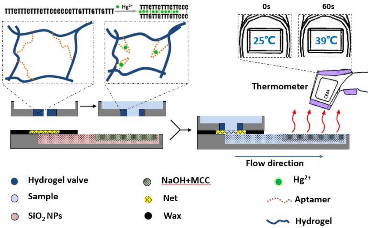
Figure S1. Schematic illustration of sampling part and euthermic part of the exothermic chip for Hg 2+ detection. MCC: microcrystalline cellulose.
