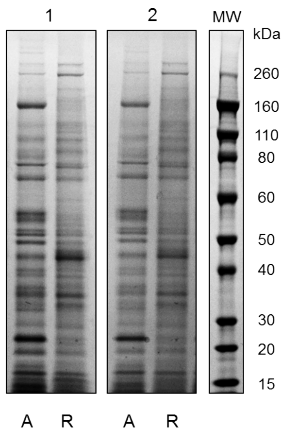
ESI, Fig. S2 – MD protein profiles before and after delipidation. NuPAGE4-12%/CBB staining of ANK and RCC MD proteins 1) before delipidation (loading 10 \mu g based on BCA protein assay) and 2) after delipidation, loading equal aliquots of both samples, considering a theoretical protein content of 10 \mu g. A = ANK; R = RCC.
