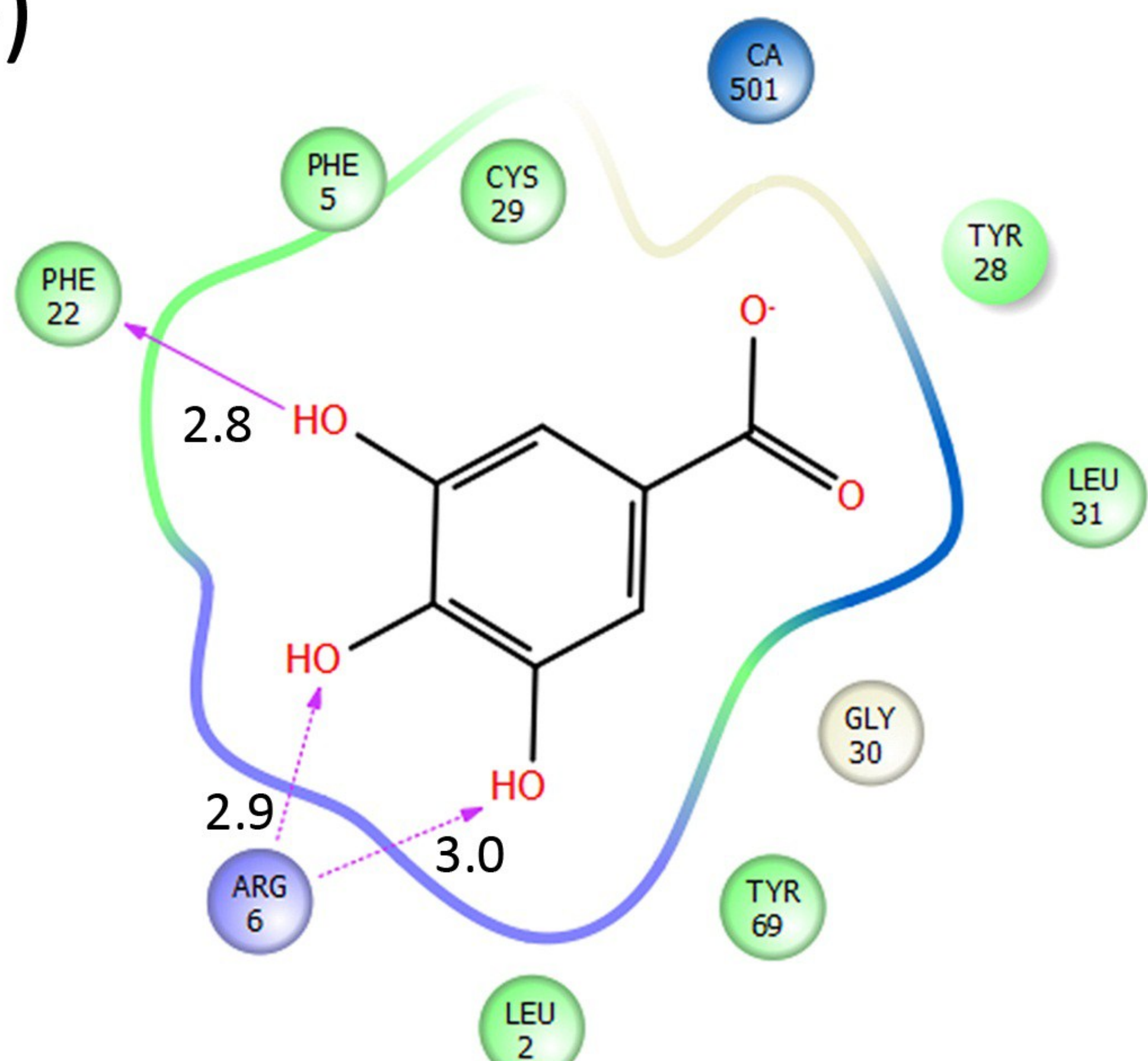
Gallic acid
