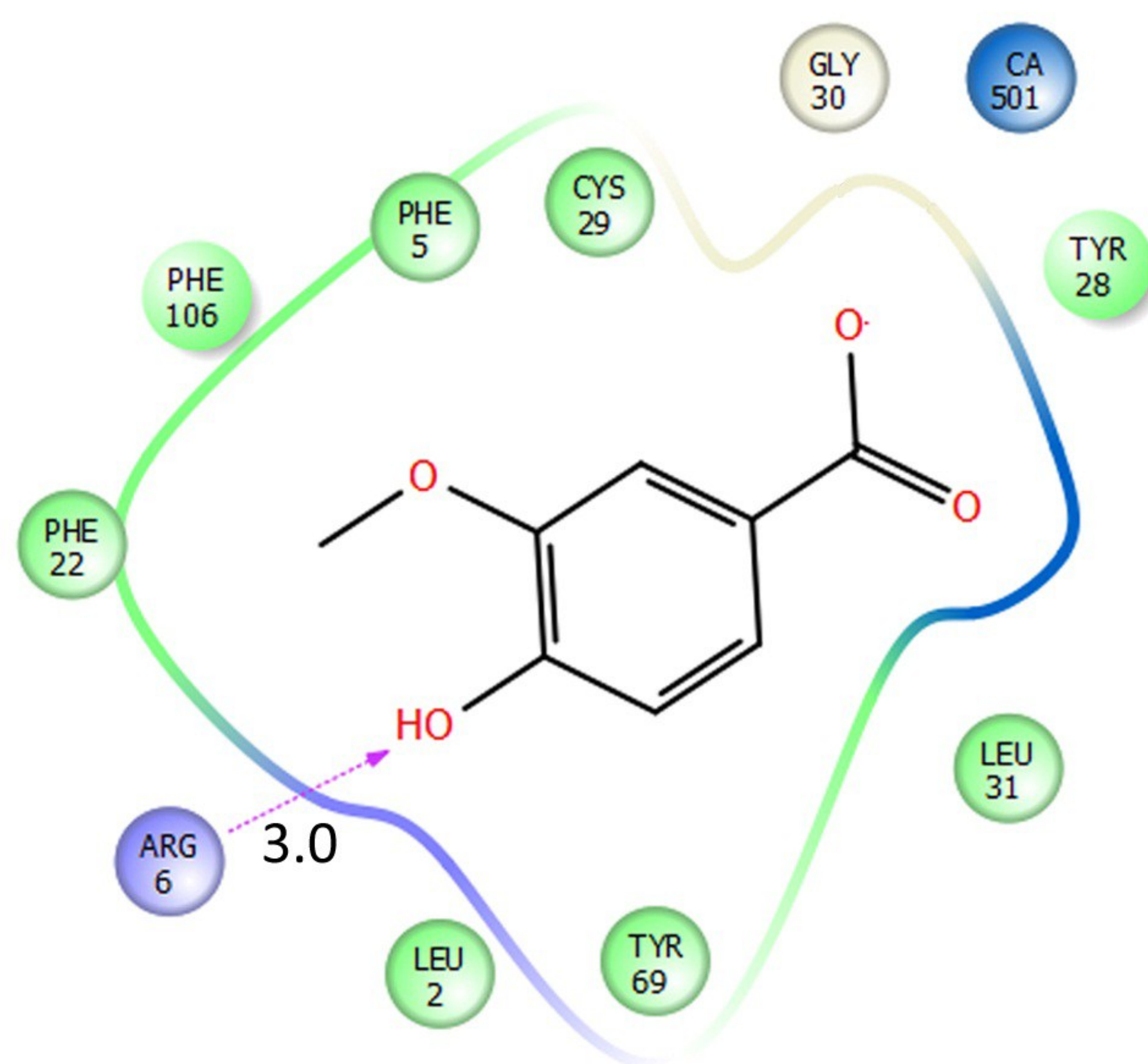
Vanillic acid
