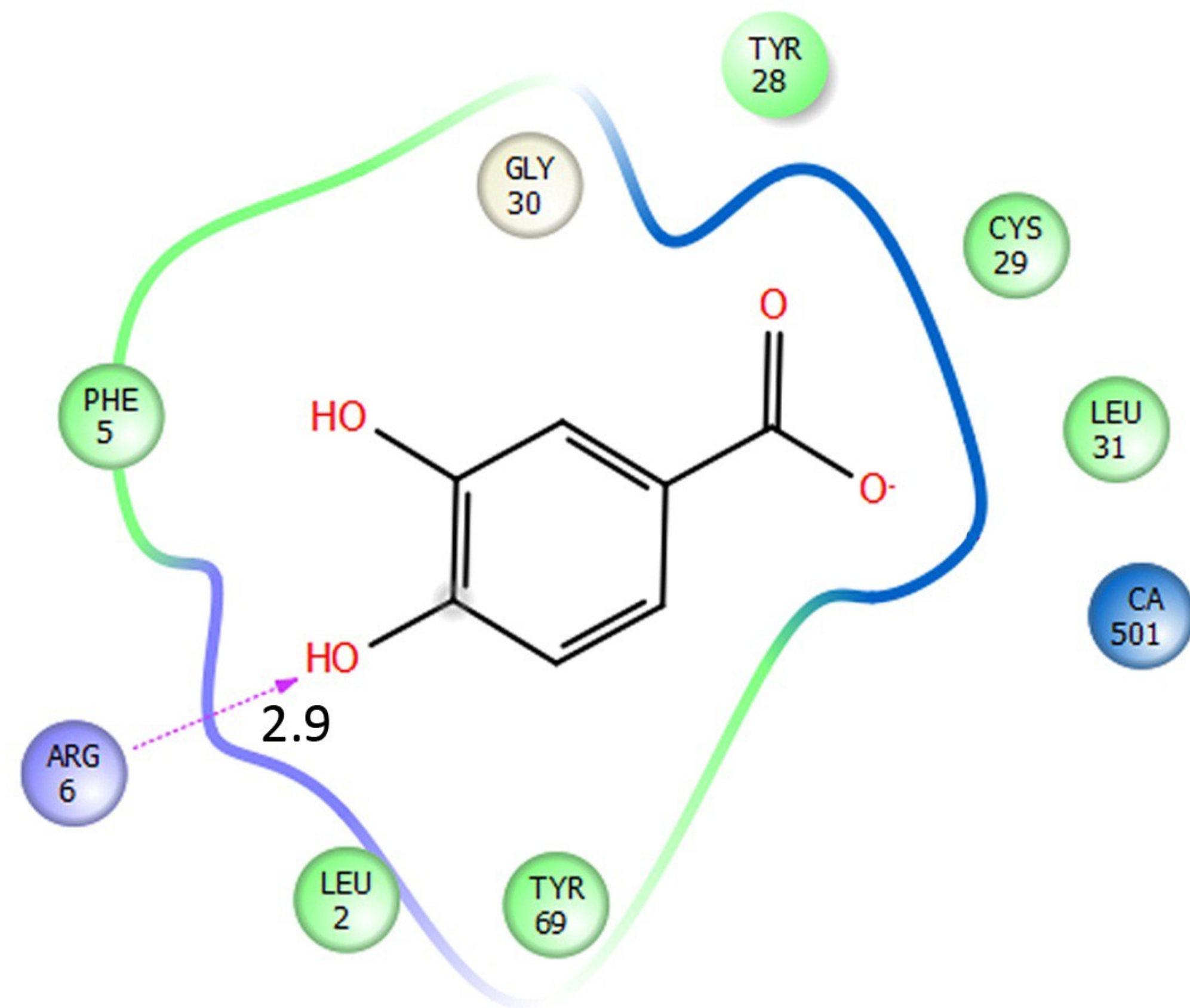
Protocatechuic acid
