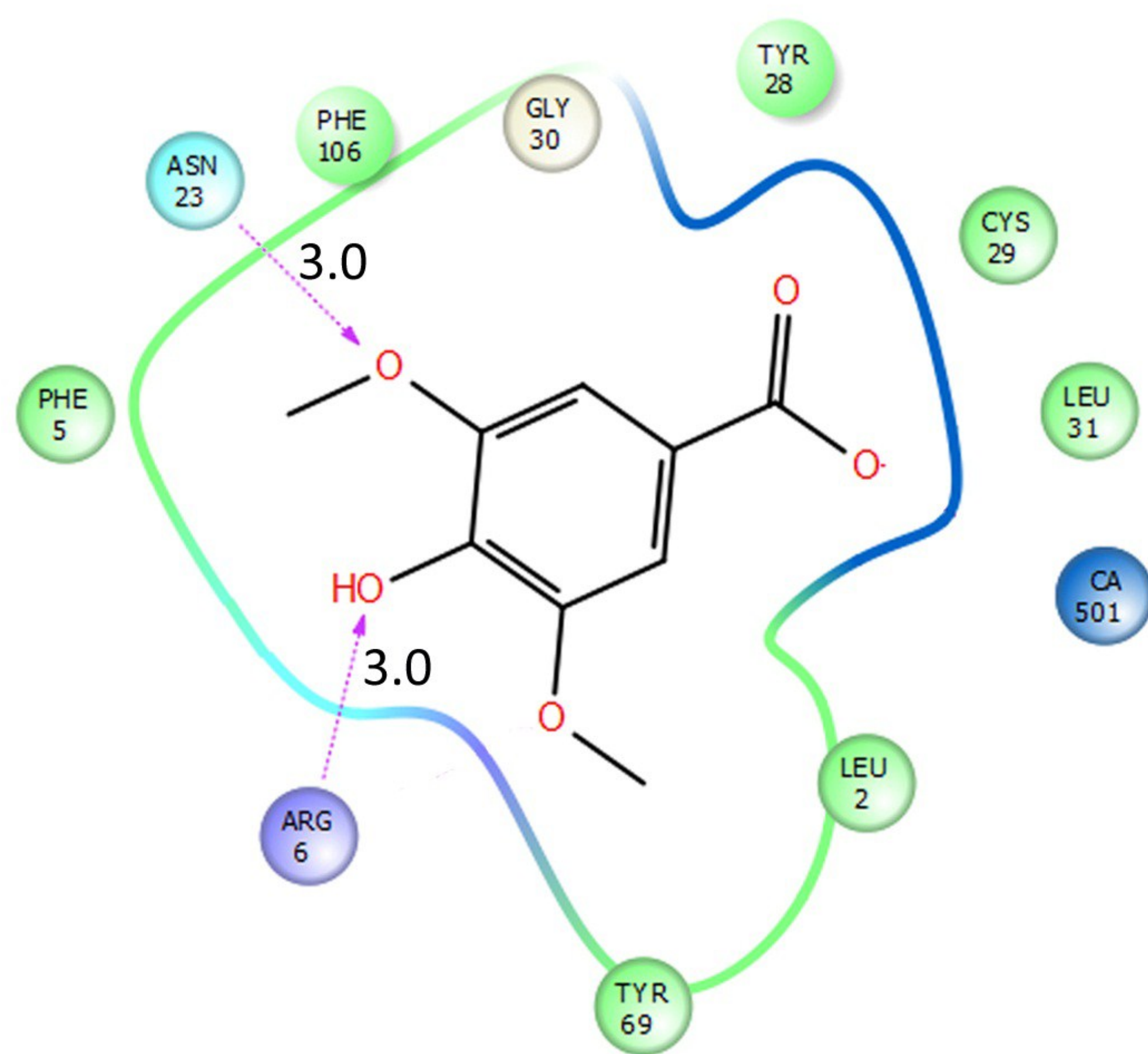
Syringic acid
