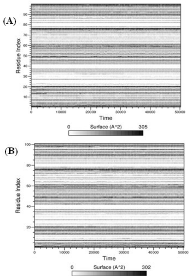
Fig. 1 Accessible surface area of the WT-β2m (A) and its mutant D76N (B) during 50 ns simulation period
