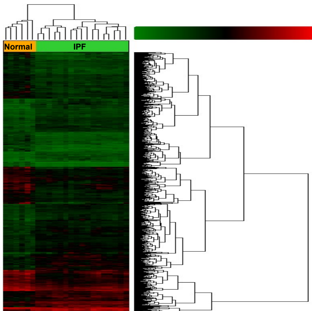
Figure S1 Hierarchical Cluster analysis of four IPF datasets.
