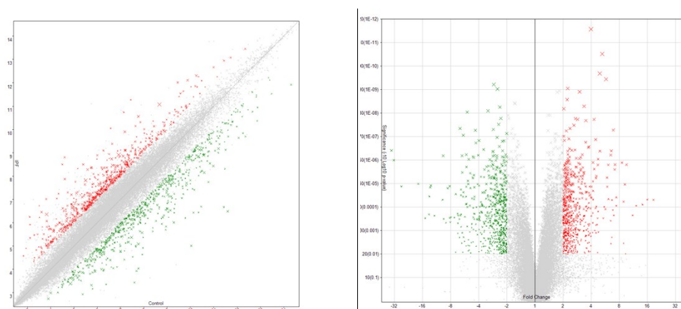
Figure S2 Scatter plot and Volcano plot of differential expression genes.
