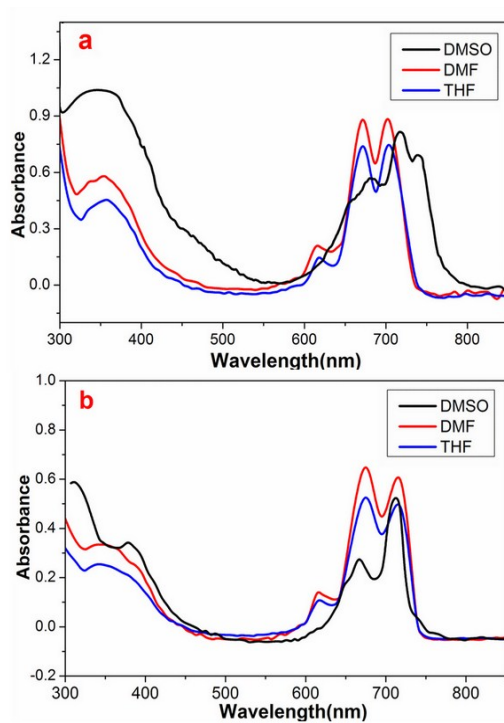
Fig.S1. Electronic absorption spectra of TBIT-Pc (a) and TBTT-Pc (b) in DMSO, DMF and THF. The measured concentration is 2.5 \times 10^{-5} M.
