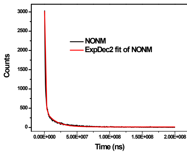
Fig. S2 Phosphorescence decays of NONP and NONM at 40 K.
