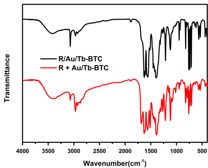
Figure S1 FT-IR spectra of R + Au/Tb-BTC and R/Au/Tb-BTC.
