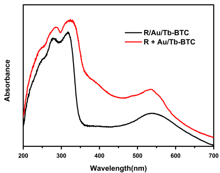
Figure S2 UV-vis spectra of R + Au/Tb-BTC and R/Au/Tb-BTC.
