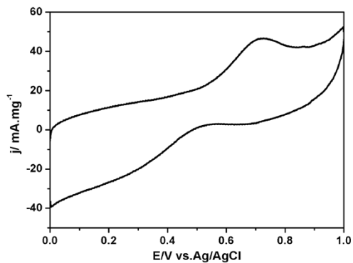
Figure S3. CV curves of MCNPs/Pt without using ionic liquid as stabilizer at the scan rate of 50 \text{ mV s}^{-1} in (0.5 \text{ M H}_2\text{SO}_4)/(0.5 \text{ M CH}_3\text{OH}) aqueous solution.
