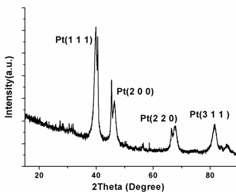
Figure S1. XRD patterns of MCNPS/Pt.
