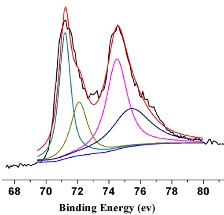
Figure S4. Pt 4f XPS spectra of MCNPs/Pt.
