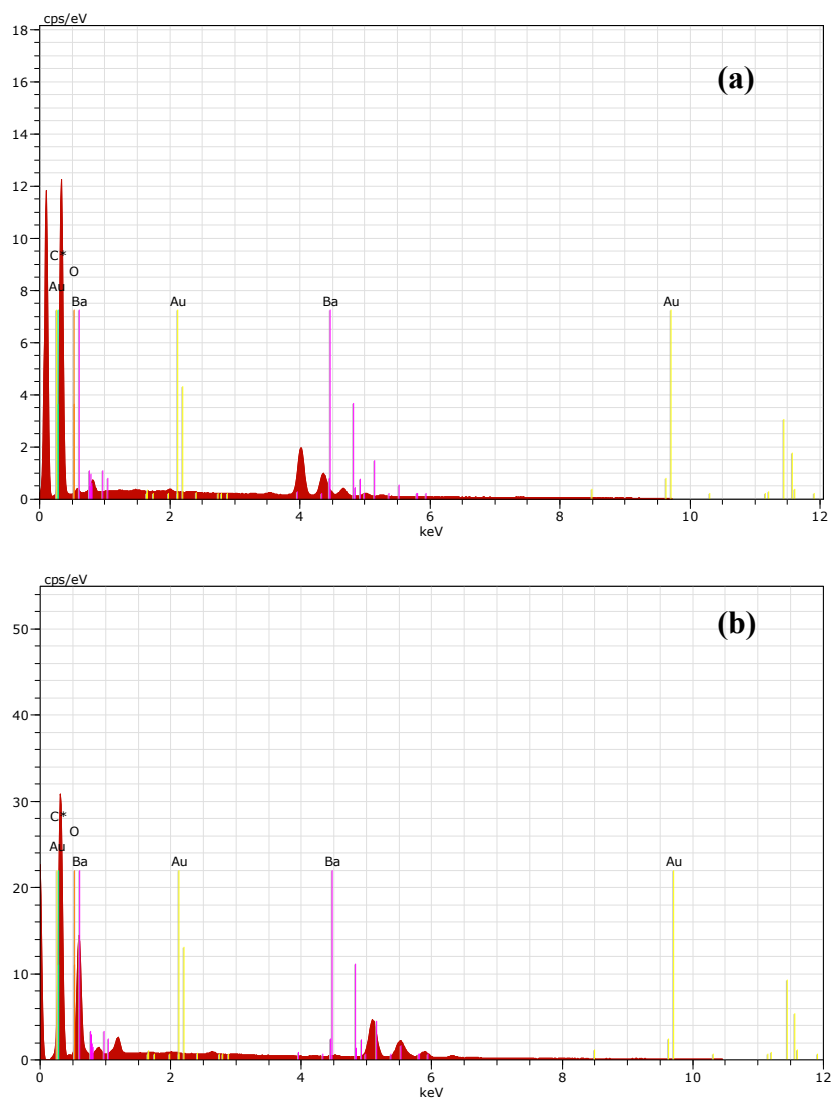
Fig. S2 SEM-EDAX spectrum of Au-NPs based Composite gels: (a) Ba/Alg/CMC/Au (b) Ba/Alg/CMC/GO/Au
