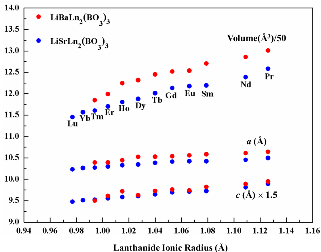
Figure S1. Plot of a , c and unit-cell volume of \text{LiMLn}_2(\text{BO}_3)_3 compounds versus \text{Ln}^{3+} ionic radius.
