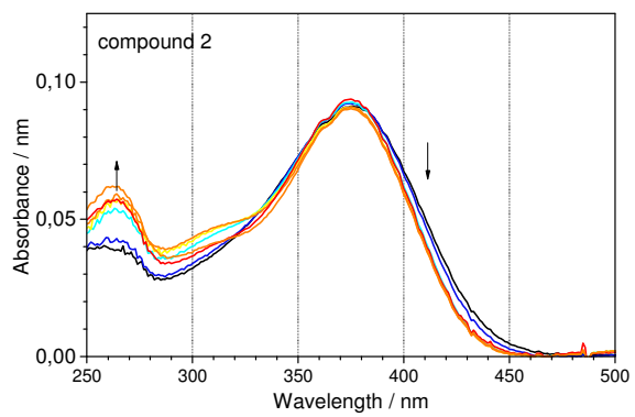
Figure S1 UV-Vis spectra recorded during oxidation of compounds 1 and 2 in \text{CH}_2\text{Cl}_2/\text{Bu}_4\text{NPF}_6 solution.
