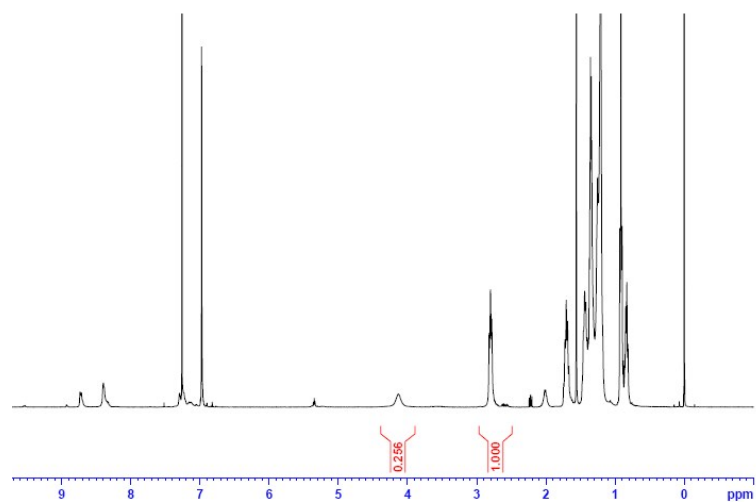
Figure S5. ^1\text{H} NMR spectra of BCP2-2.
