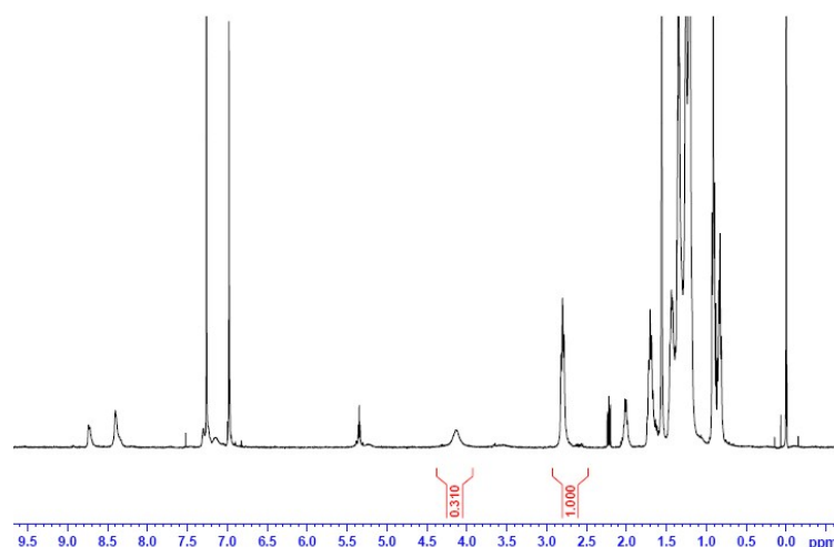
Figure S1. 1 H NMR spectra of BCP1-1.
