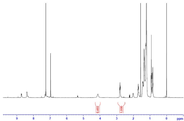
Figure S3. ^1\text{H} NMR spectra of BCP1-3.
