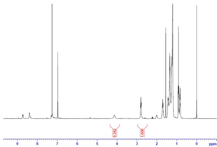
Figure S6. ^1\text{H} NMR spectra of BCP2-3.
