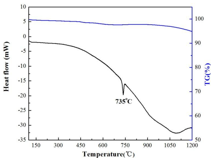
Figure S2. The DSC-TG curves for \text{Ca}_3\text{Nd}_3(\text{BO}_3)_5 .
