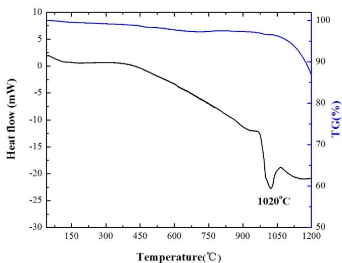
Figure S1. The DSC-TG curves for \text{Cd}_4\text{NdO}(\text{BO}_3)_3 .
