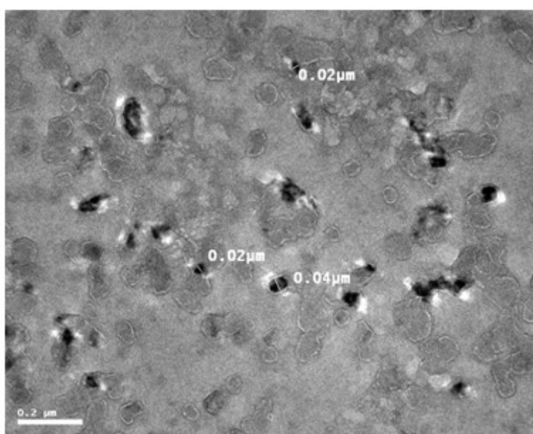
Figure S1: TEM image of the TiO 2 /PAM core/shell nanocomposite.
