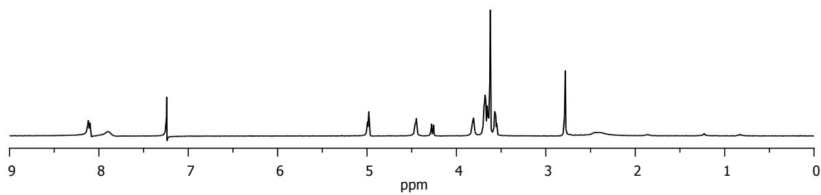
Fig. S1. ^1\text{H} NMR Spectrum of benzoic acid fullerene bis adducts (BAFB) compound
