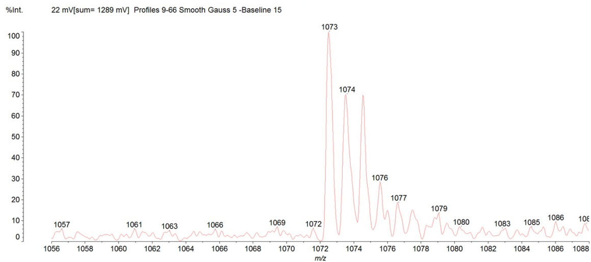
Fig. S3. Mass spectra of benzoic acid fullerene bis adducts (BAFB) compound
