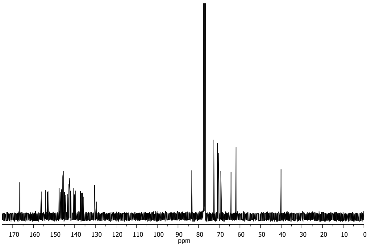
Fig. S2. ^{13}\text{C} NMR Spectrum of benzoic acid fullerene bis adducts (BAFB) compound
