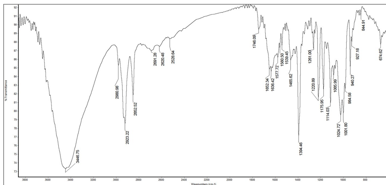
IR spectrum of 1-cyclohexylpiperazinedithiocarbamic acid
