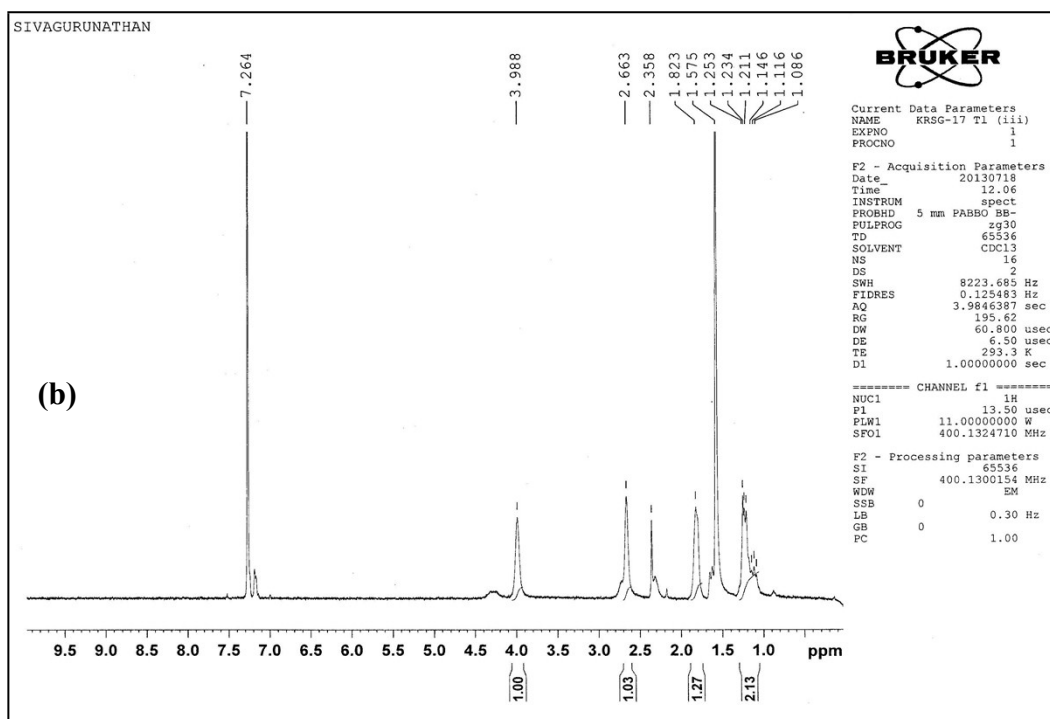
^1\text{H} NMR Spectra of (a) [\text{Ti}(\text{chpzdtc})_2] and (b) [\text{Ti}(\text{chpzdtc})_3]
