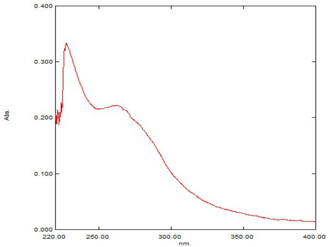
UV spectrum of 1-cyclohexylpiperazinedithiocarbamic acid
