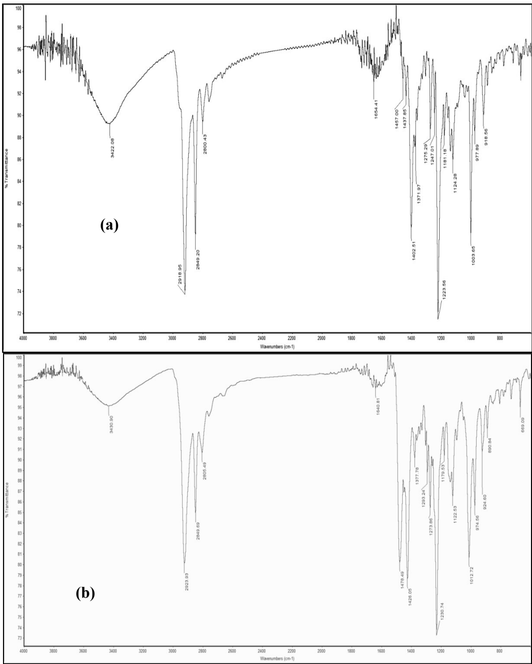
IR spectra of (a) [Ti(chpzdtc)]_2 and (b) [Ti(chpzdtc)_3]
