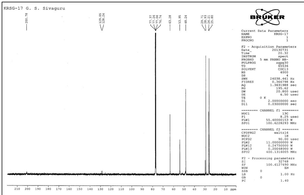
^{13}\text{C} NMR Spectrum of [\text{Tl}(\text{chpzdtc})_3]
