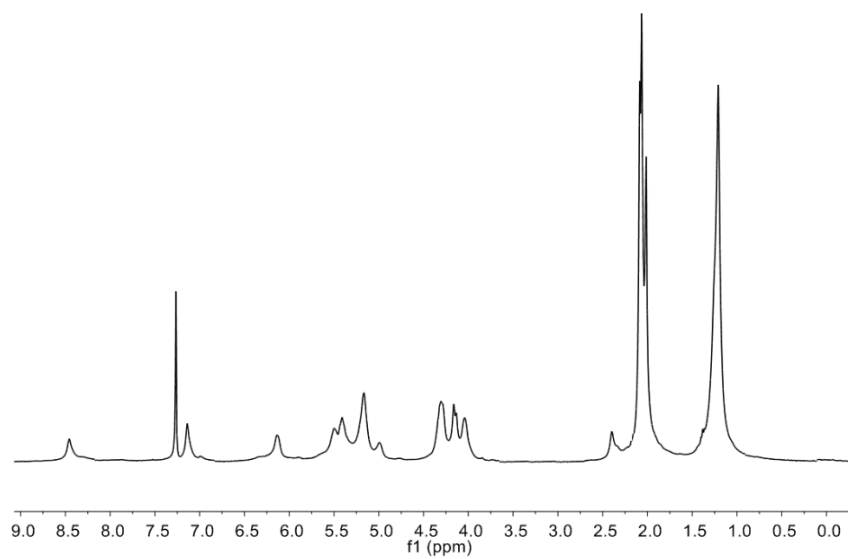
^1\text{H} NMR spectrum of TrpGH-OAc
