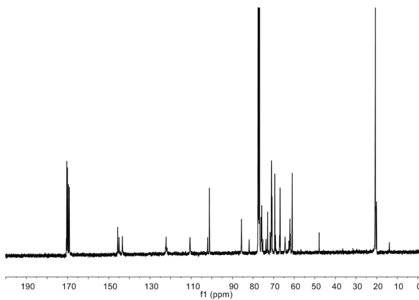
^{13}\text{C} NMR spectrum of TrpL-OAc
