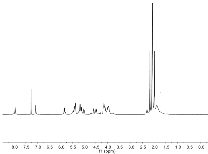
^1\text{H} NMR spectrum of TrpL-OAc
