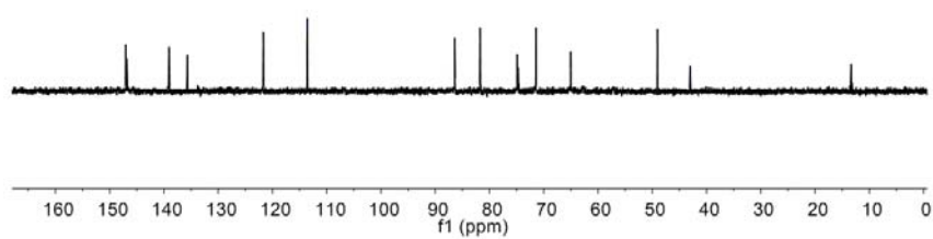
^{13}\text{C} NMR spectrum of TrpGH
