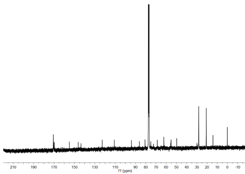
^{13}\text{C} NMR spectrum of TrpGH-OAc
