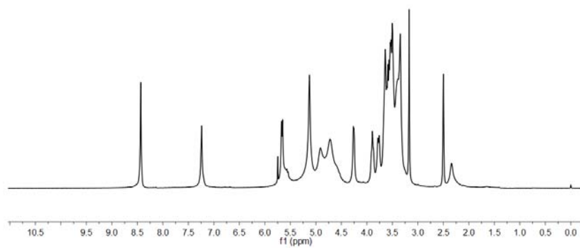
^1\text{H} NMR spectrum of TrpL
