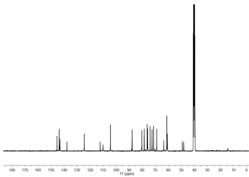
^{13}\text{C} NMR spectrum of TrpL
