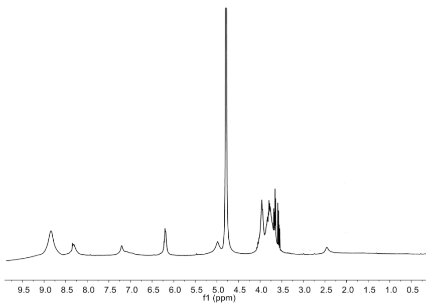
^1\text{H} NMR spectrum of TrpGH
