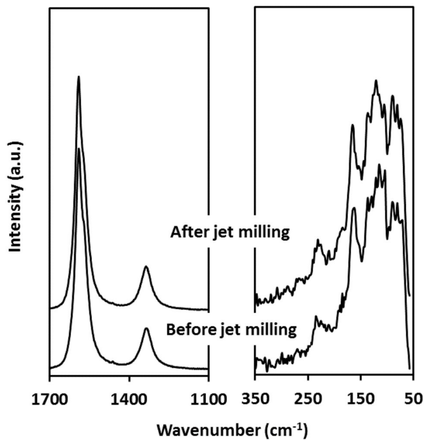
Fig. S1 Raman spectra measured from the heat&current SWCNTs before/after jet milling.
