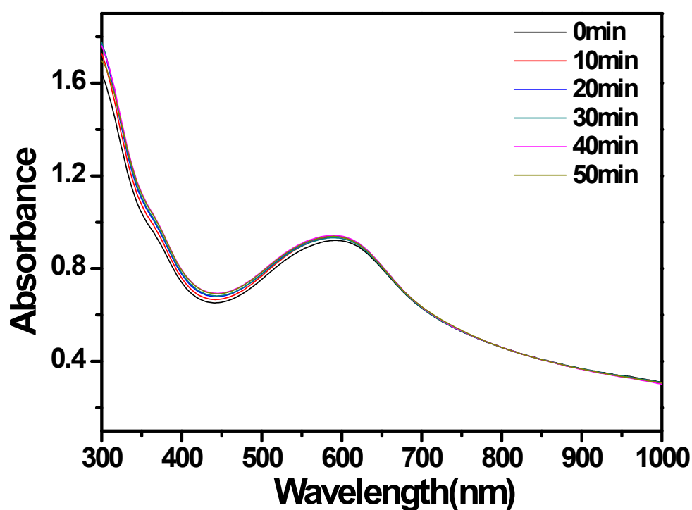
Supporting Figure S1. UV-vis-NIR absorbance spectra of the \text{TiS}_2 -PEG solution before and after irradiation by the 808-nm laser at the power density of 0.8 \text{ W/cm}^2 for different periods of time. \text{TiS}_2 -PEG showed great stability under a long period of photothermal heating.
