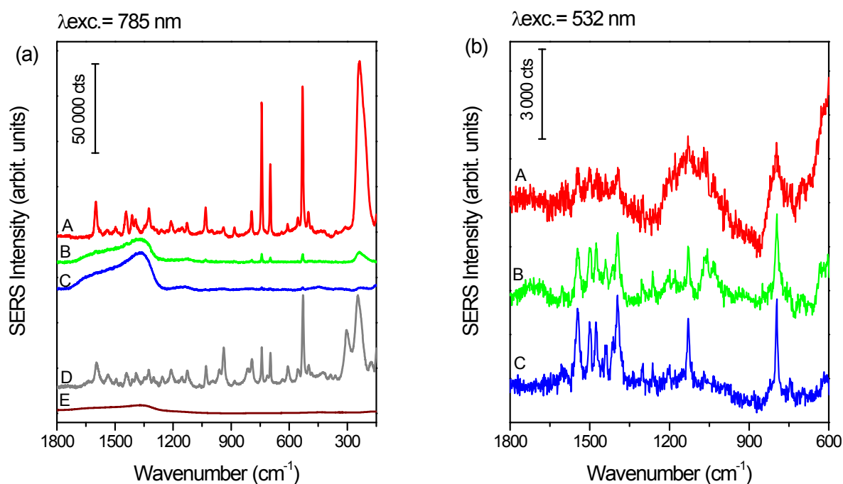
Figure S1: SERS spectra of ThT (1 μM) on different colloids substrates at two different excitation wavelengths: a) 785 nm and b) 532 nm.
