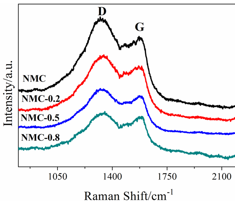
Fig. S1 Raman spectra of the NMC- x .
