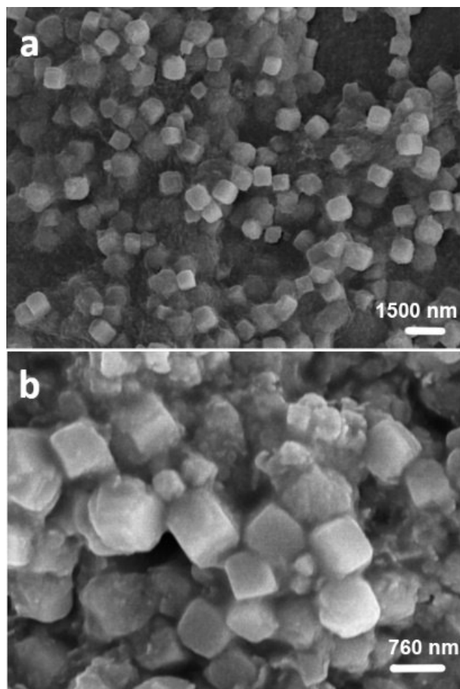
Figure S2. a, and b) SEM images of as-prepared samples after 10000 cycles of electrochemical testing.
