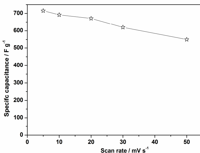
Figure S1. The plot of specific capacitance vs. scan rate for as-prepared MHCF nanocube electrode.
