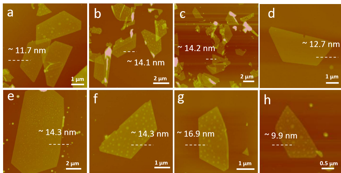
Fig. S1 Complementary AFM profiles of thin SnSe 2 NSs.
