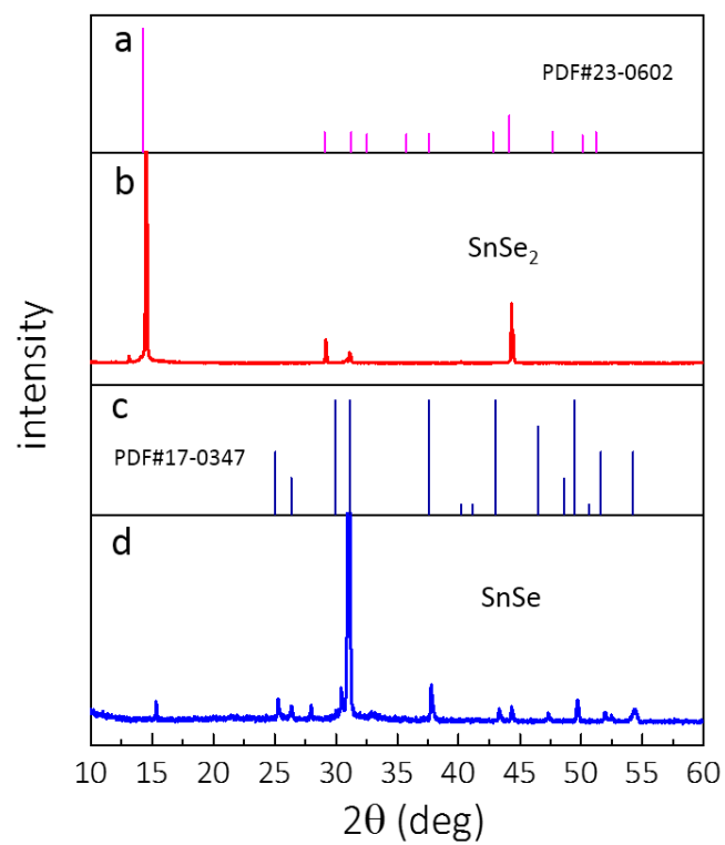
Fig. S2 XRD data of (a) standard \text{SnSe}_2 (b) as grown \text{SnSe}_2 NSs (c) standard \text{SnSe} and (d) as grown \text{SnSe} NSs.
