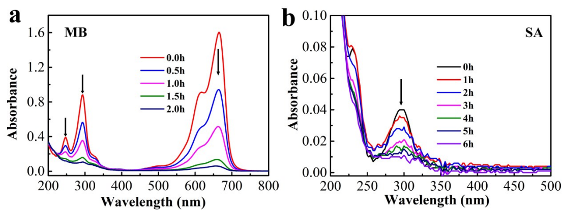
Fig. S4. UV-Vis absorption spectra of (a) MB and (b) SA solutions with ZMS/AuNPs-3 as a function of irradiation time.
