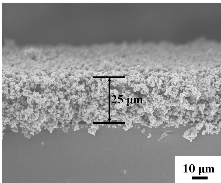
Fig. S1. Cross sectional SEM image of as-prepared ZMS/AuNPs film.
