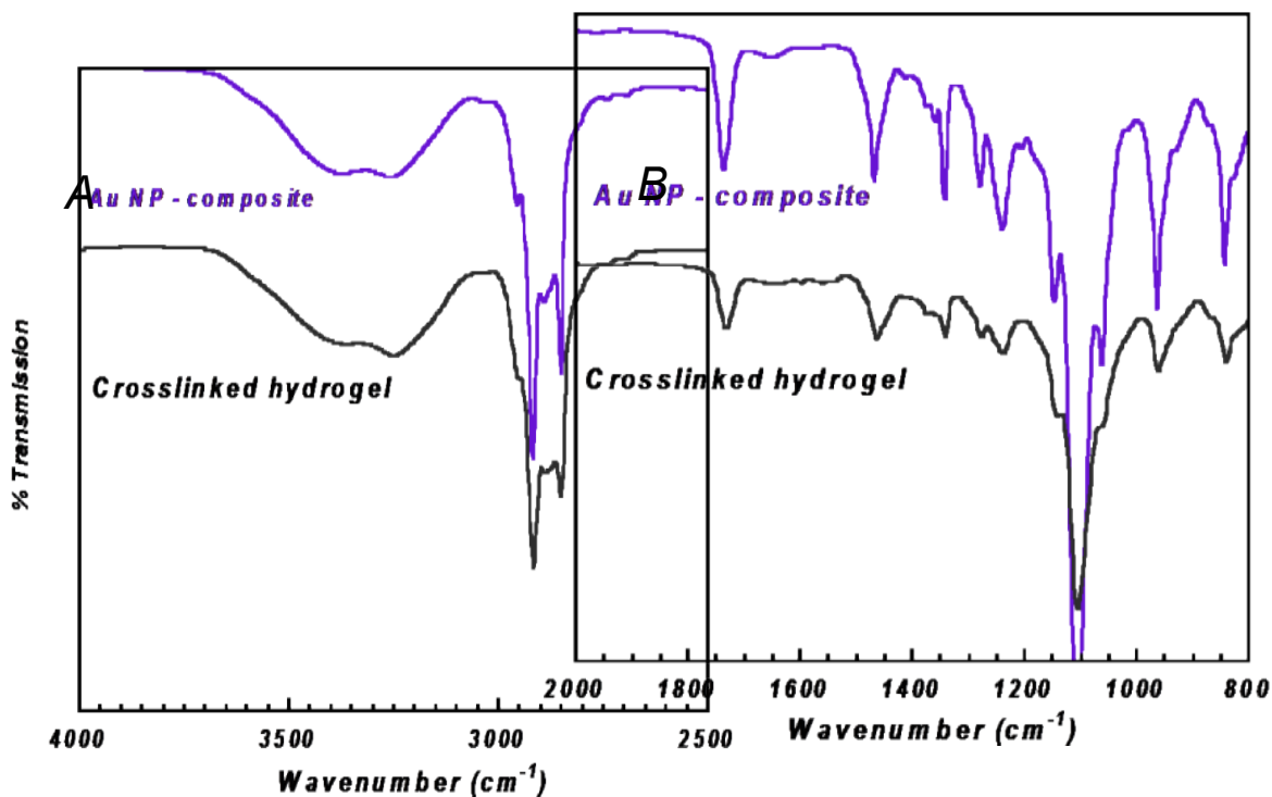
Figure S1. Comparison of ATR/FTIR spectra collected on photoinitiated crosslinked F98(Acr) 2 -based complex fluid (black curve) to Au-NP composite (purple curve). (A) high frequency region and (B) low frequency region.
