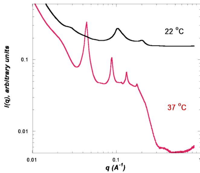
Figure S2. Temperature dependent SAXS profiles collected on the mesophase prior to gelation.
