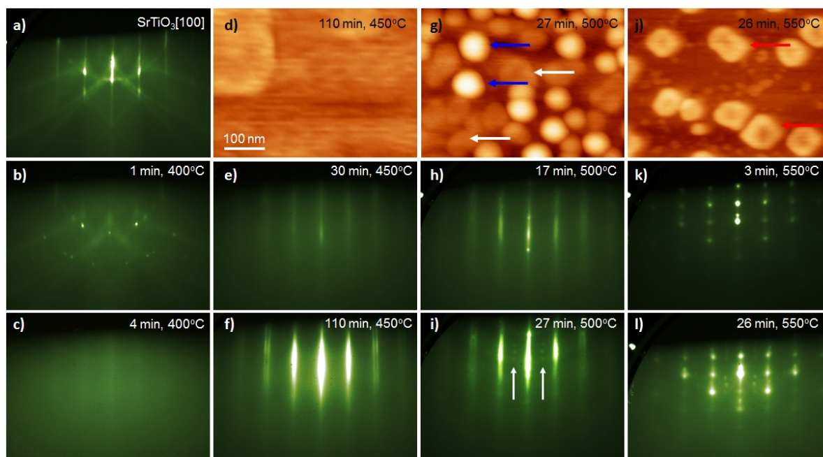
Figure s1: RHEED patterns taken along [100] azimuthal direction and AFM images (d, g, and j) of \text{MoO}_3 films grown on \text{SrTiO}_3(001) . Total deposition time and substrate temperature for each film are marked.
