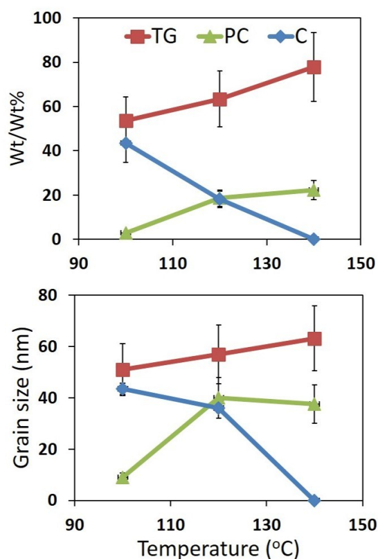
Figure S1. Grain size and TG, PC and C perovskite phases wt/wt% growth, calculated from XRD data of perovskite treated with MAI at various temperatures.
