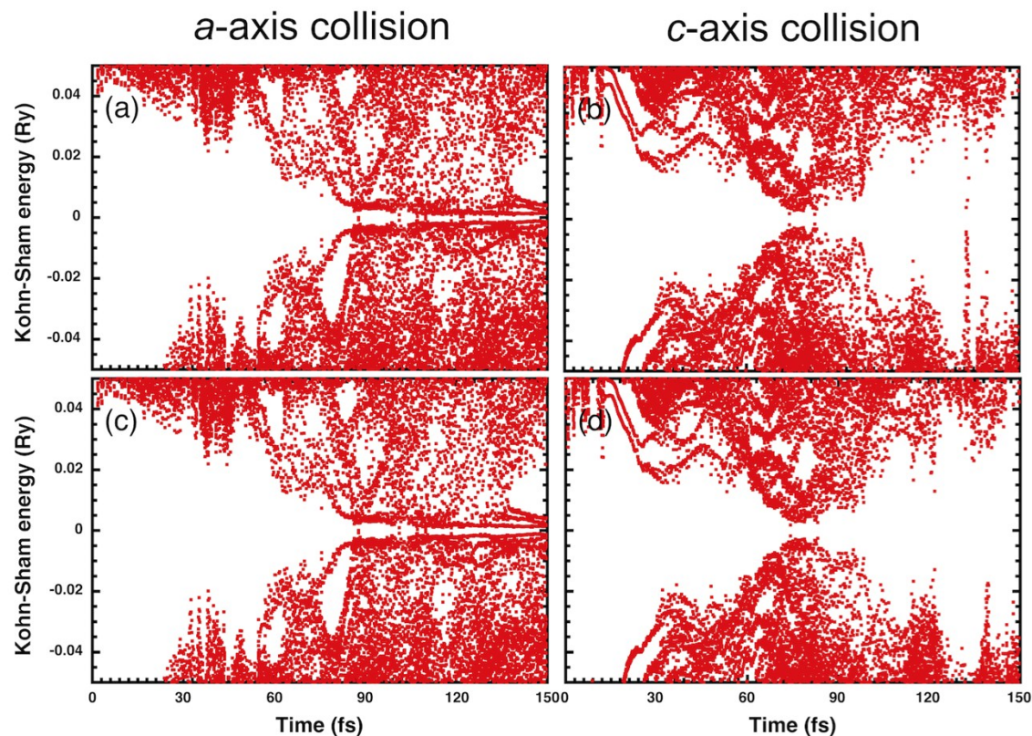
Fig. S1. Kohn-Sham eigenenergies as a function of time (a) and (c) for the 6 km/s a -axis collision of two additional trajectories, (b) and (d) for the 6 km/s c -axis collision of another two additional trajectories.
