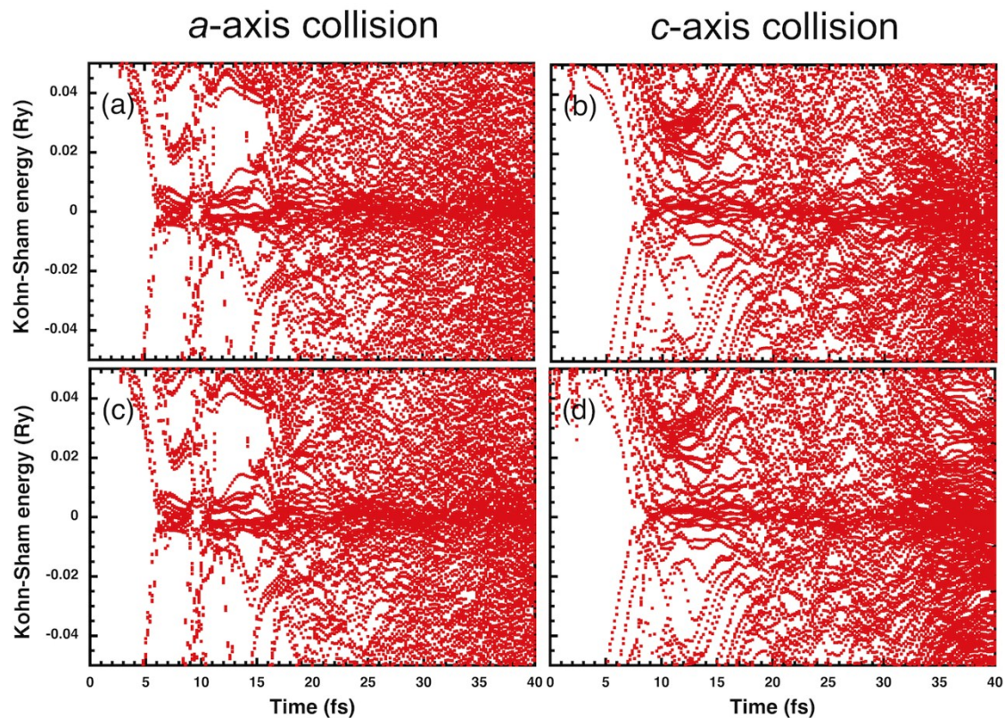
Fig. S2. Kohn-Sham eigenenergies as a function of time (a) and (c) for the 20 km/s a -axis collision of two additional trajectories, (b) and (d) for the 20 km/s c -axis collision of another two additional trajectories.
