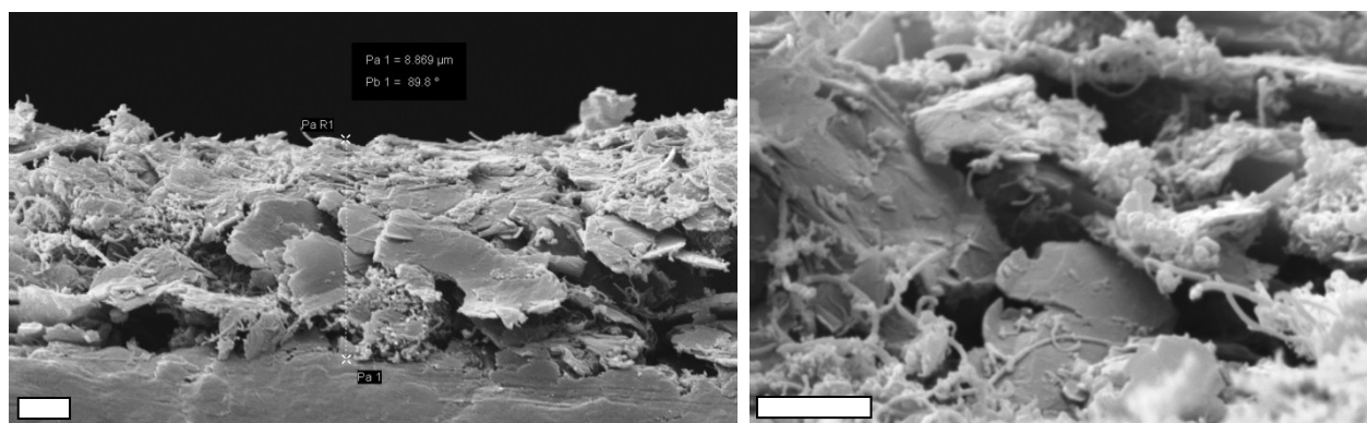
Fig. S1. Characteristic SEM images of the hybrid pG/MWNT-f-OH thin films from the cross sectional area before compression. The measured mean thickness is about 9 μm. The bars are 2 μm.
